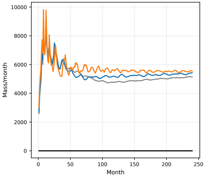
(a) Mean \pm 95% CI
