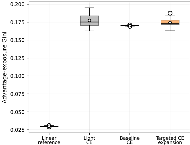
Spatial-advantage exposure inequality: last 24 months
