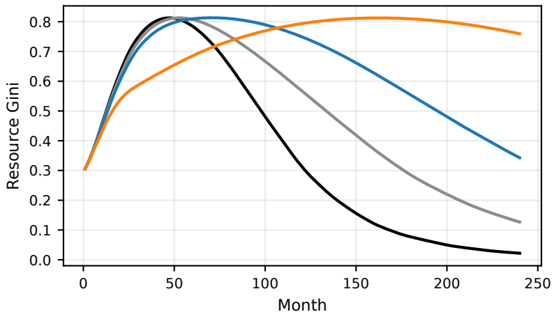
Accumulated economic-resource inequality
