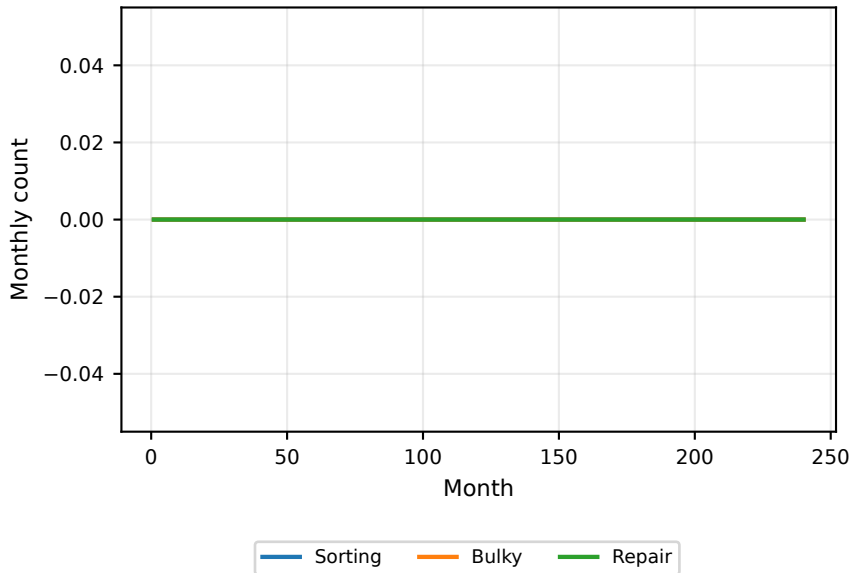
K3 flow decomposition: Linear reference
