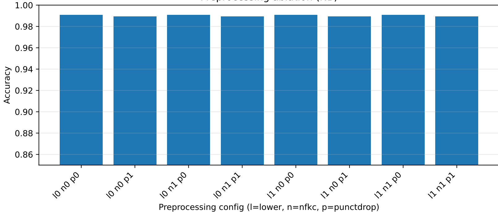
Preprocessing ablation (NB)
