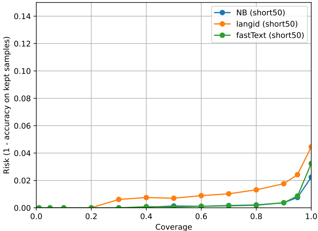
Coverage-Risk (short50)
