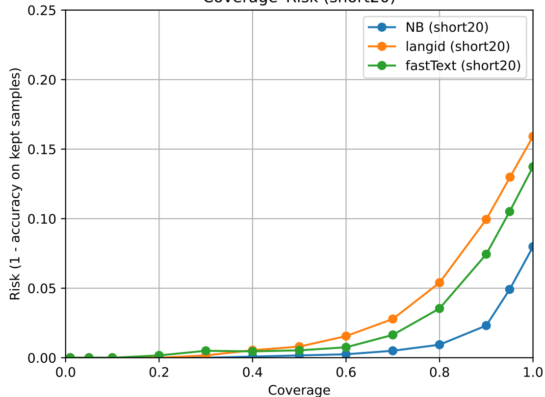
Coverage-Risk (short20)
