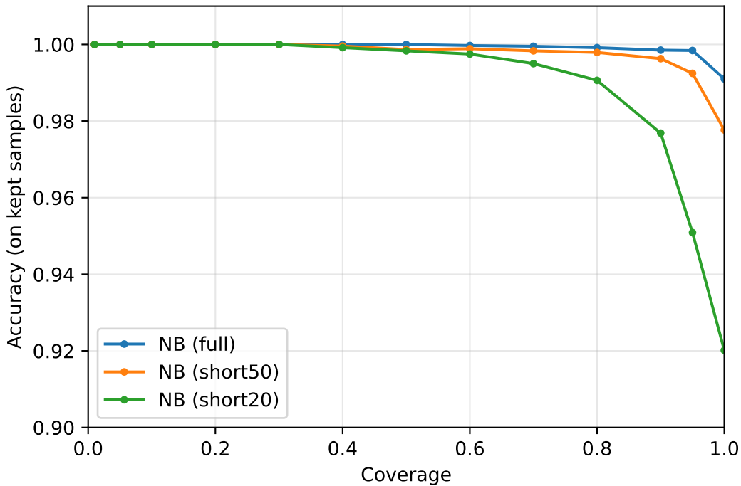
NB selective prediction (ngram-normalized margin)
