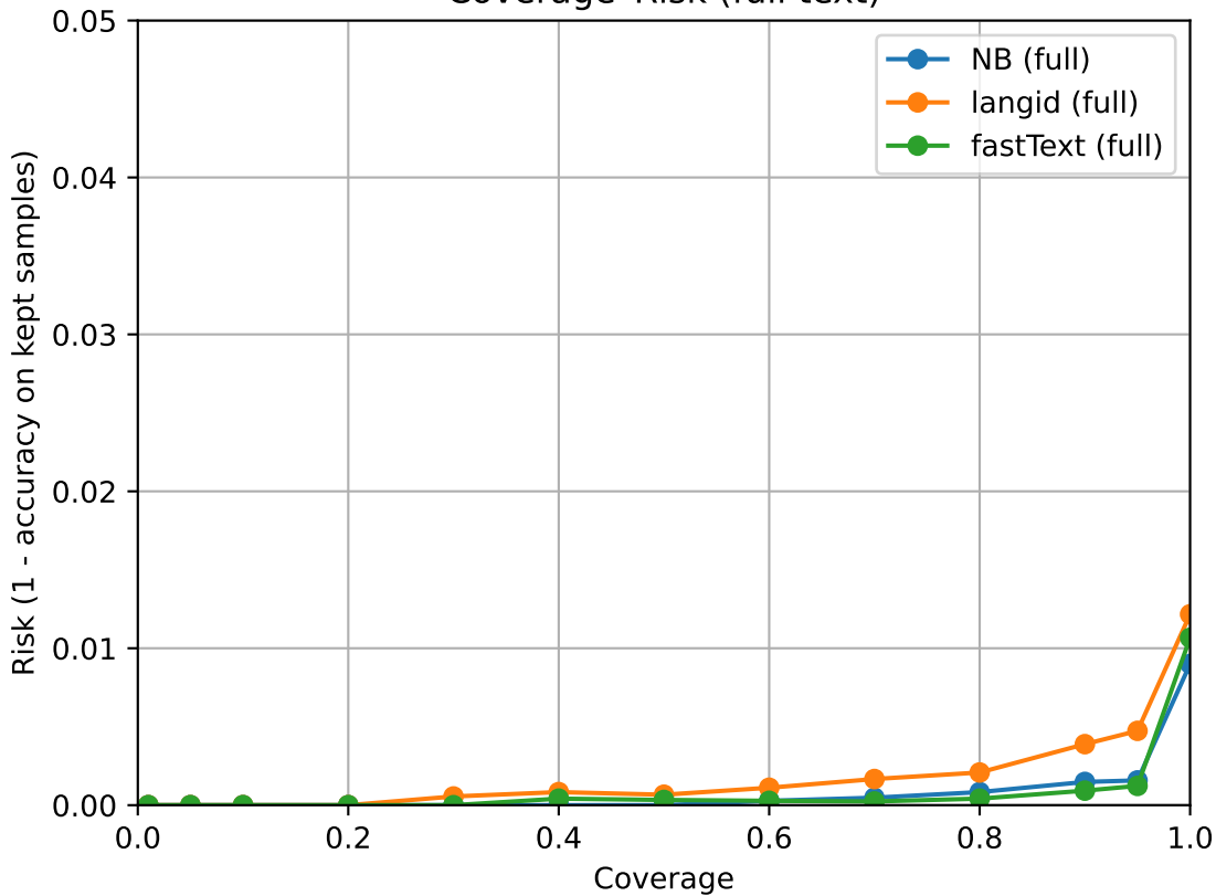
Coverage-Risk (full text)
