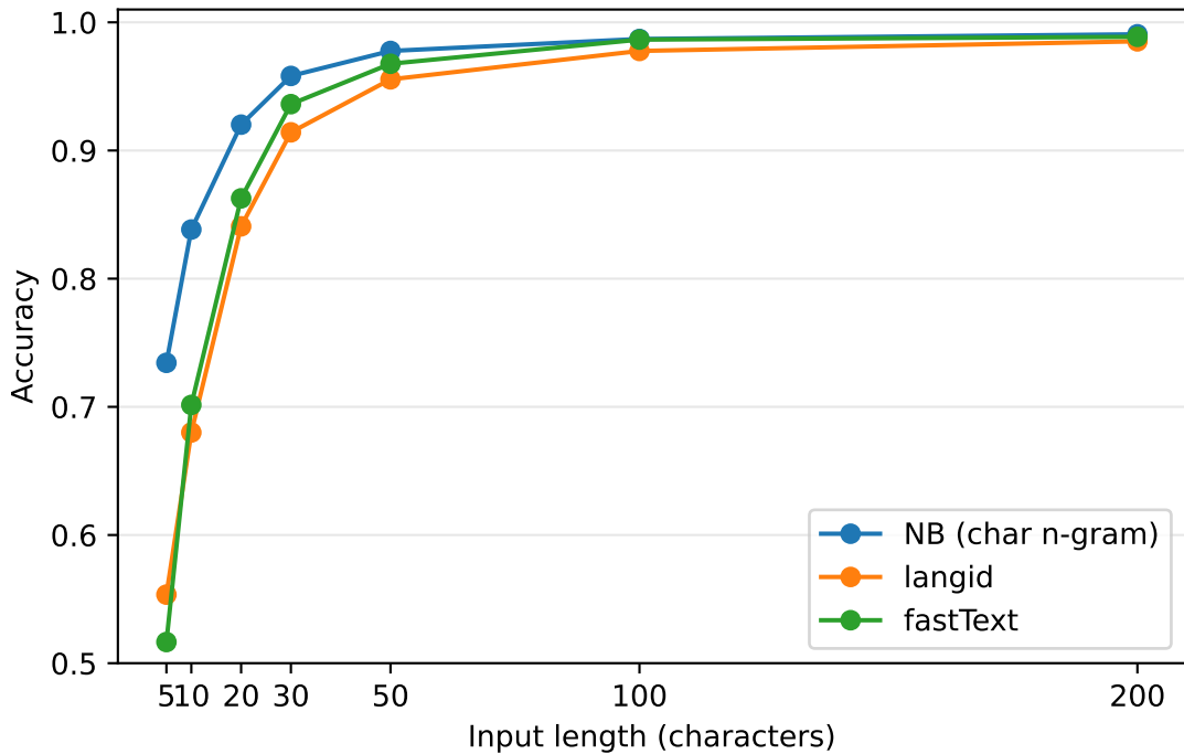
Short-text robustness
