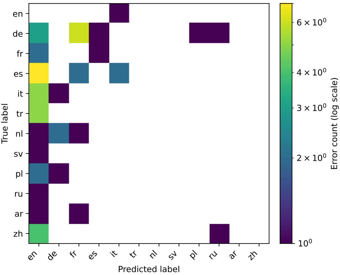
Confusion matrix (NB)
