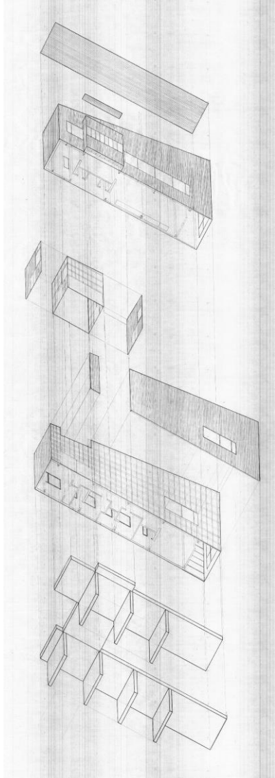
Worm's Eye View
