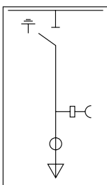
进线隔离柜
