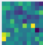
SERS map
