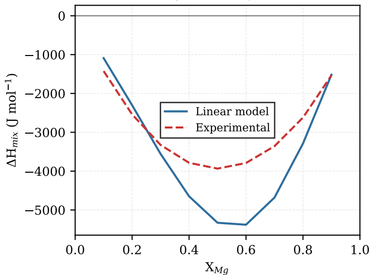
(C) Mixing Enthalpy at 1000 K
