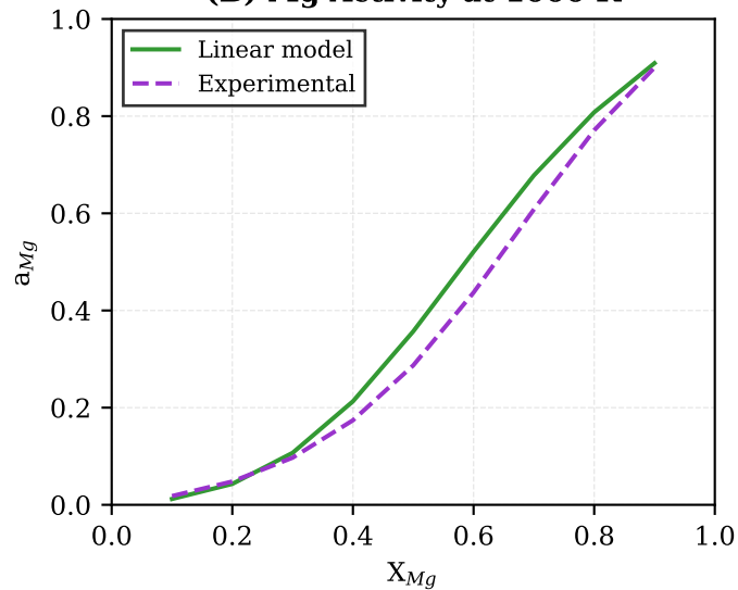
(B) Mg Activity at 1000 K
