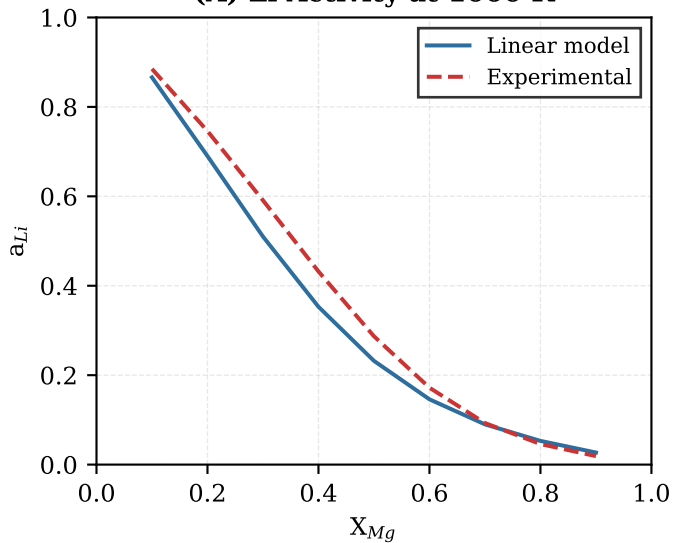
(A) Li Activity at 1000 K
