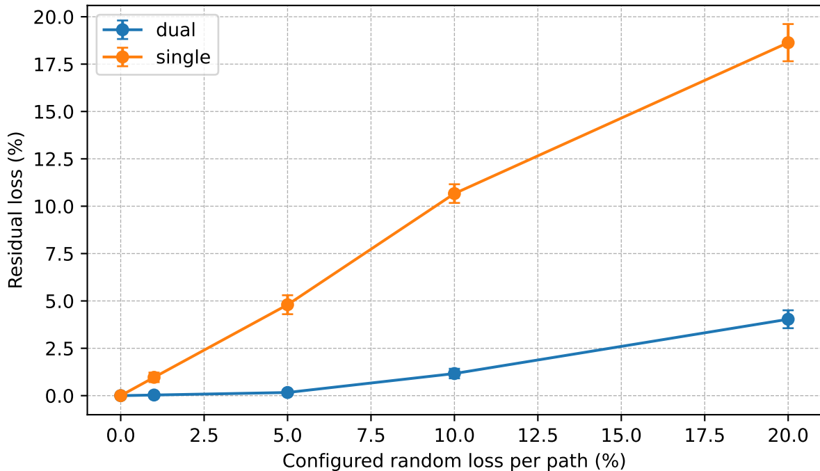
Residual packet loss
