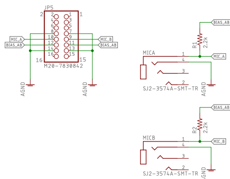
Microphone Circuit
