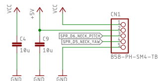
Connector Circuit for Power Board Connection
