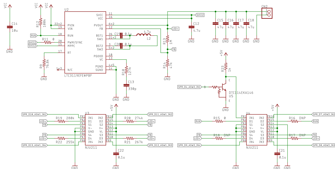
4.2V - 4.5V Adjustable Power Circuit for LED Bulb
