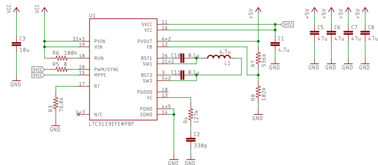
5V Power Circuit for Spresense and Servo Motors
