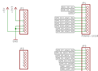
Connector Circuit for Spresense Connection
