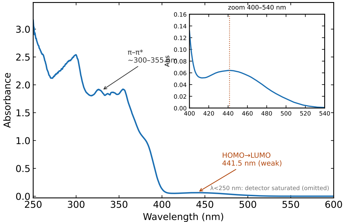
UV-vis absorption of neutral helicene (DBPO double[5]helicene)
