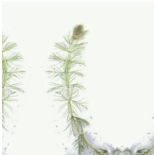
Resized Crop
