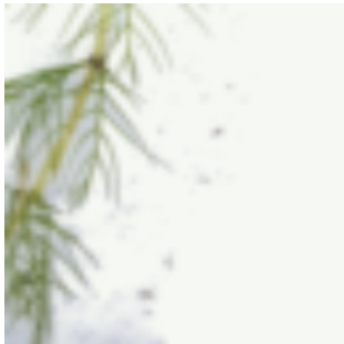
Close-up Crop
