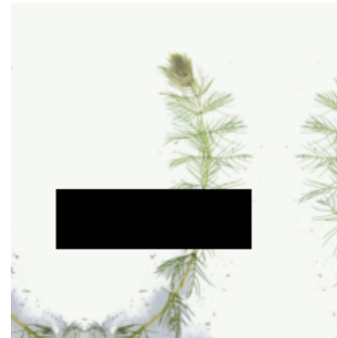
Random Erasing
