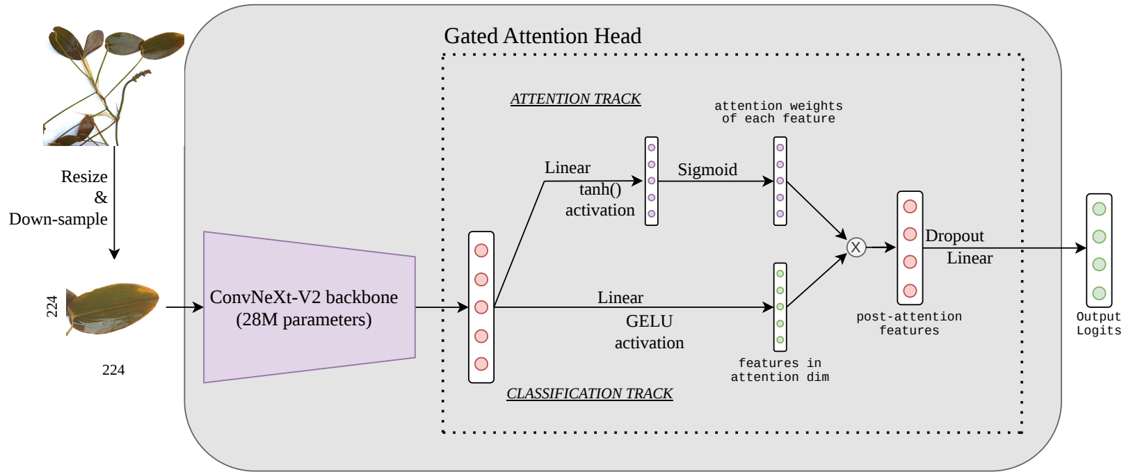
1. Classification Model
