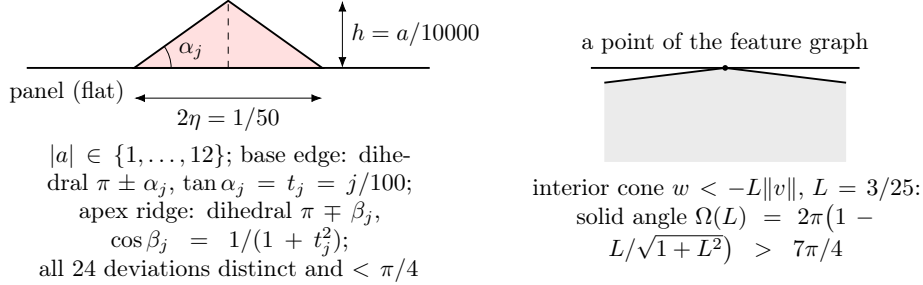
FIGURE 13. Schematic feature geometry, with exaggerated height: a pyramid of height j/10000 , base half-width 1/100 , its deviation angles, and the interior cone with slope bound L = 3/25 used in Section 4.
