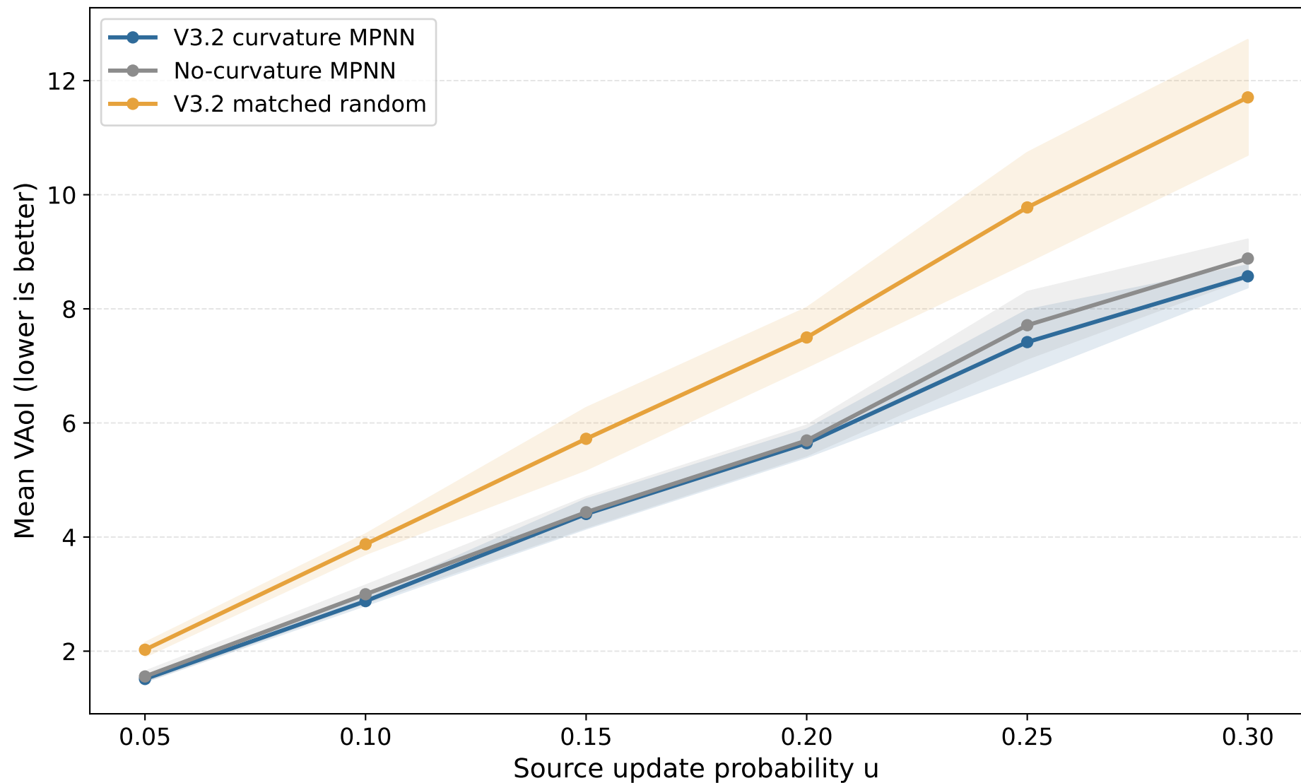
Community topology update-probability generalization
