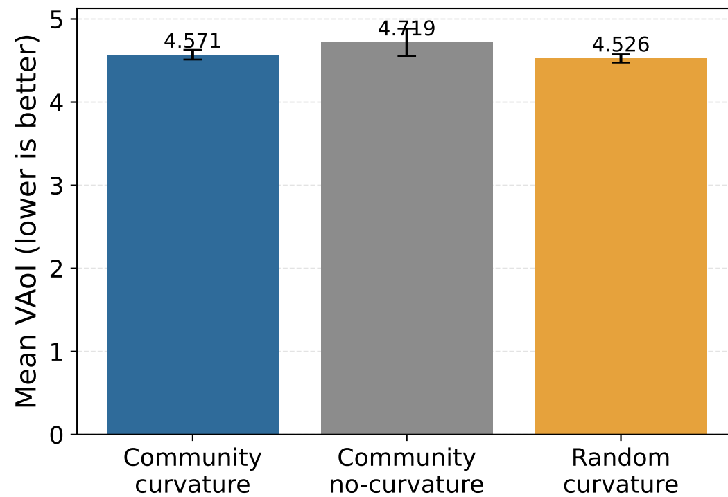
Aggregate comparison Reduction vs no-curvature: community 3.1%, random 4.1%
