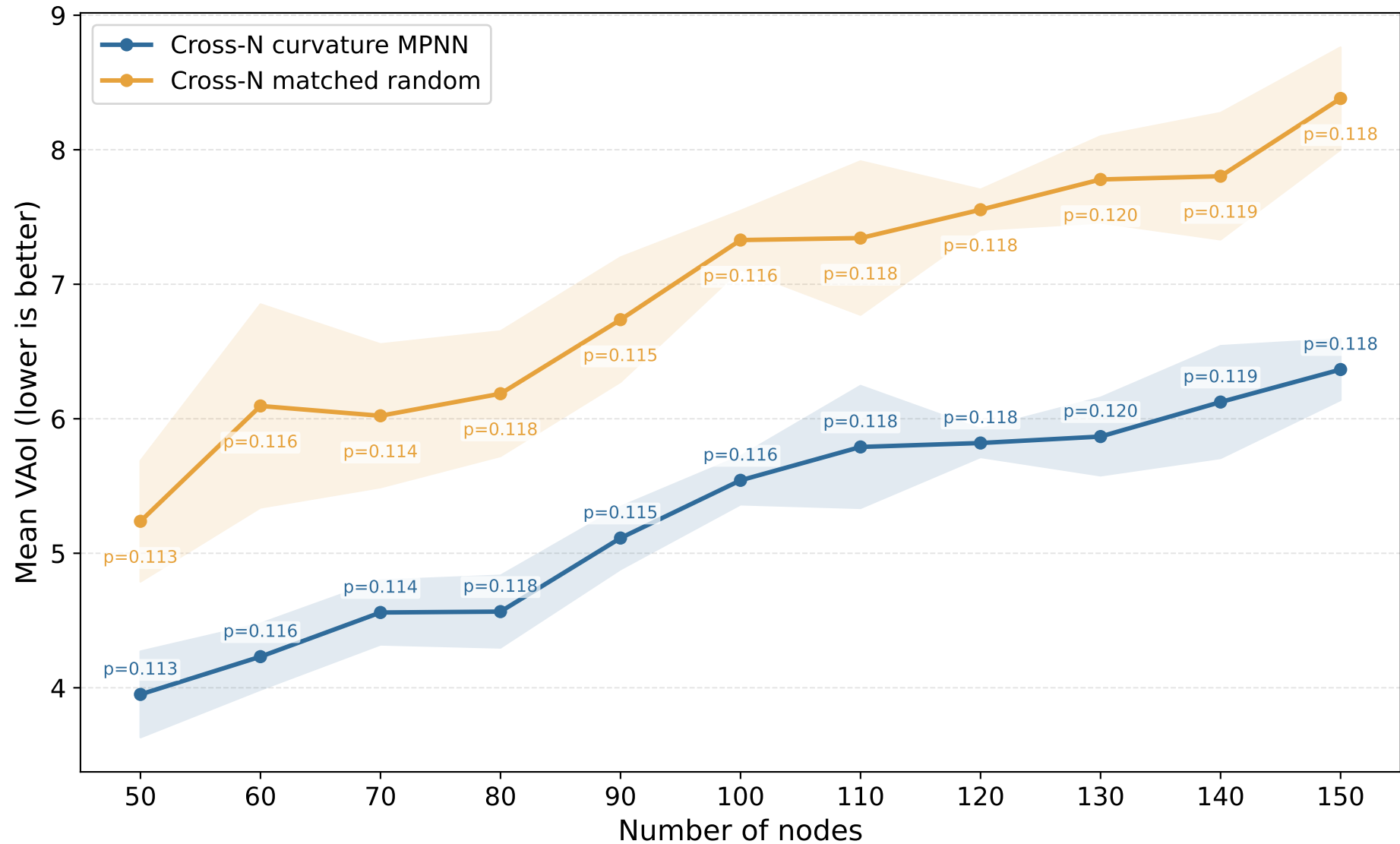
Community topology cross-N scalability generalization
