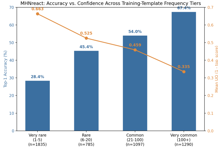
Figure 18: MHNreact: top-1 accuracy (left axis) and mean UQ (right axis) across four training-template frequency tiers. Accuracy rises from 28.4% to 67.4%, a 39-point spread, versus LocalRetro’s 47.3-point collapse from a much smaller very-rare base rate.
