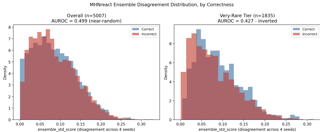
Figure 29: MHNreact ensemble disagreement distribution by correctness, overall vs. very-rare tier. The rightward shift of the “correct” distribution relative to “incorrect” in the very-rare panel is the visual signature of the inversion.
