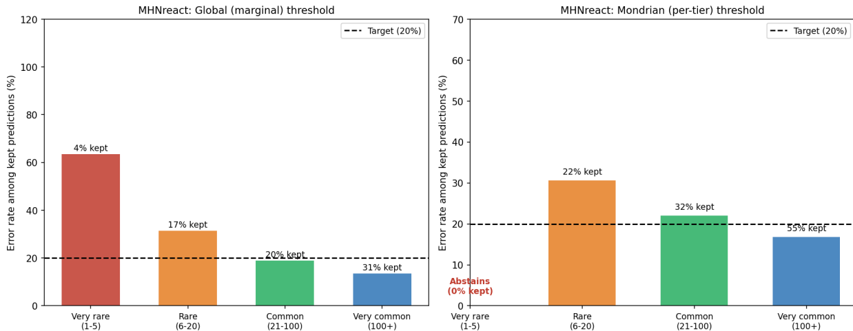
Figure 11: MHNreact selective prediction under a 20% target error rate, same harness as LocalRetro. Left : global threshold. Right : Mondrian per-tier thresholds.
