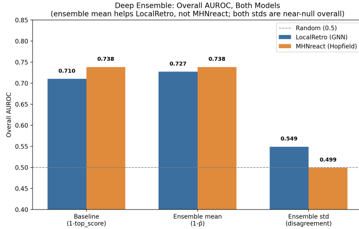
Figure 28: Deep ensemble overall (non-tiered) AUROC, both models. Ensemble mean helps LocalRetro but not MHNreact; both ensemble-std signals hover near random overall, which is why the very-rare-tier breakdown (main text Figure 9) is the figure that carries the argument.
