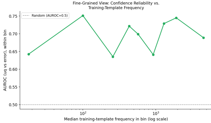
Figure 17: LocalRetro: fine grained within bin AUROC vs. median training template frequency. Reliability stays broadly stable (0.64 to 0.75) outside the most extreme rarity tail.
