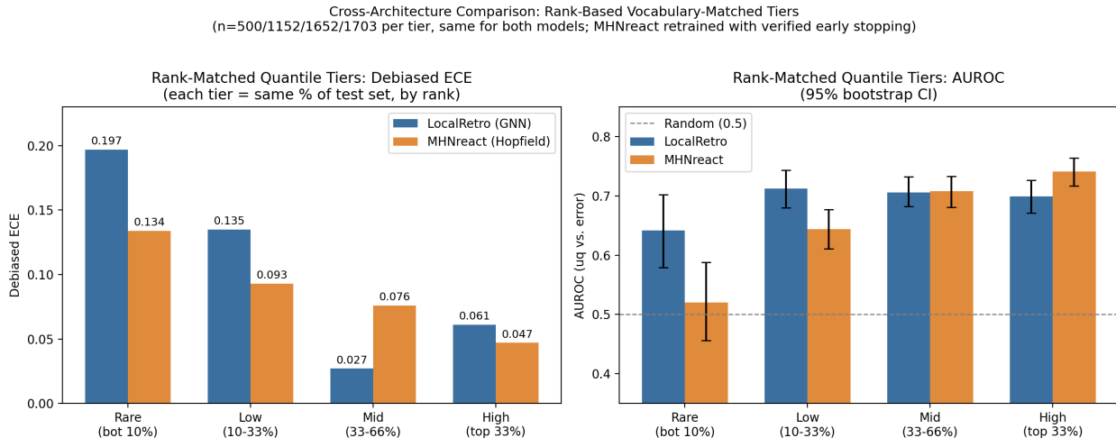
Figure 3: Rank-based vocabulary-matched tier comparison. Left : Debiased ECE by tier. Both models have highest ECE in the rare tier, but their profiles differ: LocalRetro shows a sharp drop from rare to mid (0.197 to 0.027), while MHNreact declines smoothly and monotonically (0.134 to 0.047). Right : AUROC by tier with 95% bootstrap CIs; both models maintain discrimination above random across all tiers.
