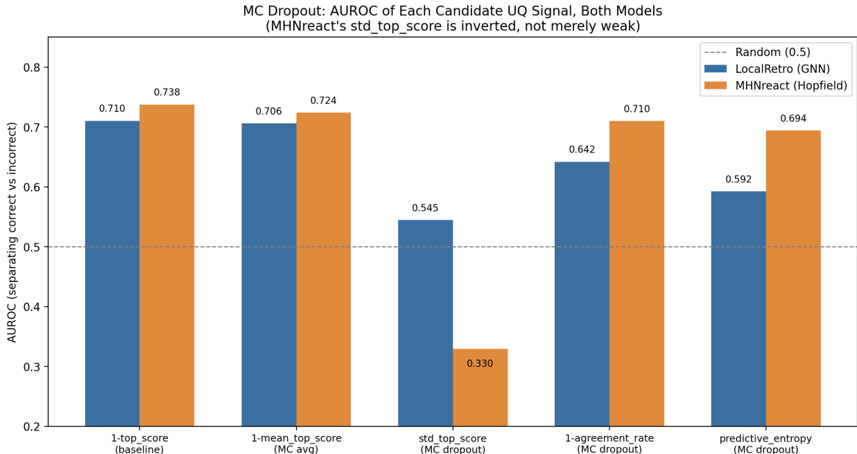
Figure 7: AUROC of each candidate MC dropout signal, both models. MHNreact’s std_top_score is not merely weak like LocalRetro’s; it is inverted, falling well below the random-chance line.
