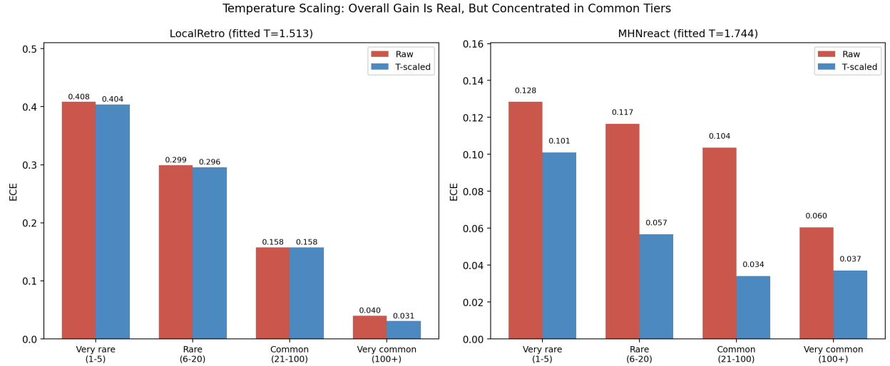
Figure 4: Temperature scaling, raw vs. T-scaled ECE by tier, both models. LocalRetro’s rare tiers barely move and the common tier is unchanged; nearly all of its overall gain comes from the very-common tier. MHNreact improves more evenly across tiers, consistent with its uniformly-miscalibrated signature rather than a sharp collapse.
