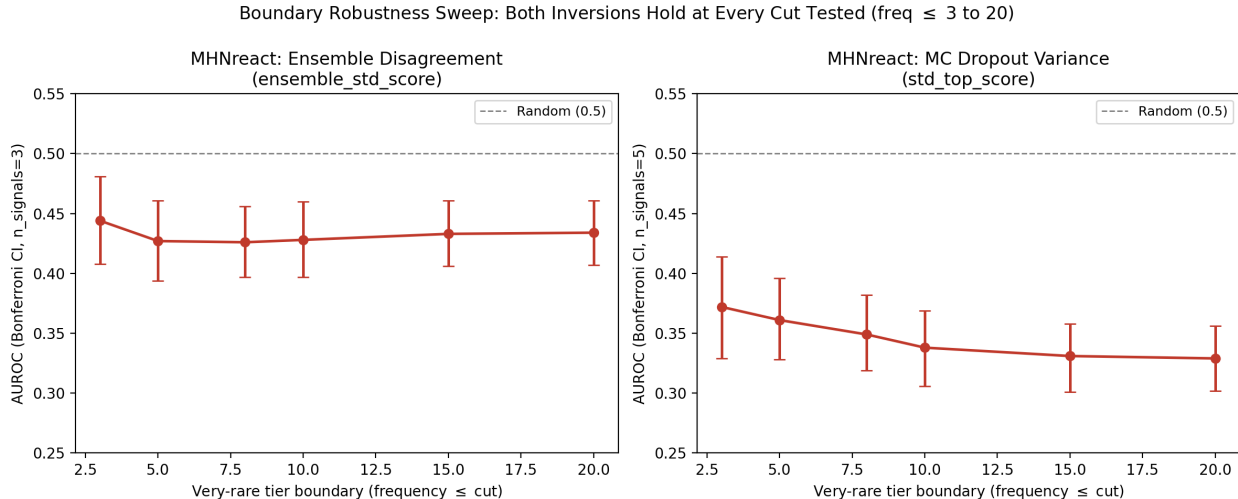
Figure 8: Boundary robustness sweep for both MHNreact inversion claims: AUROC and Bonferroni-corrected CI recomputed at six different very-rare-tier boundary definitions (freq \leq 3, 5, 8, 10, 15, 20). Both inversions (MC dropout variance, right; ensemble disagreement, left) hold at every cut tested: the CI excludes 0.5 in all six cases for both signals. A claim that holds only at one arbitrary boundary would be fragile; this one does not.
