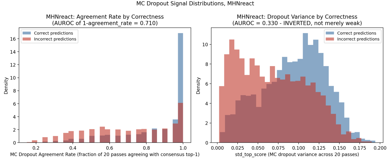
Figure 26: MHNreact: MC dropout signal distributions by correctness. Left : agreement rate. Right : dropout variance, showing the inversion visually.
