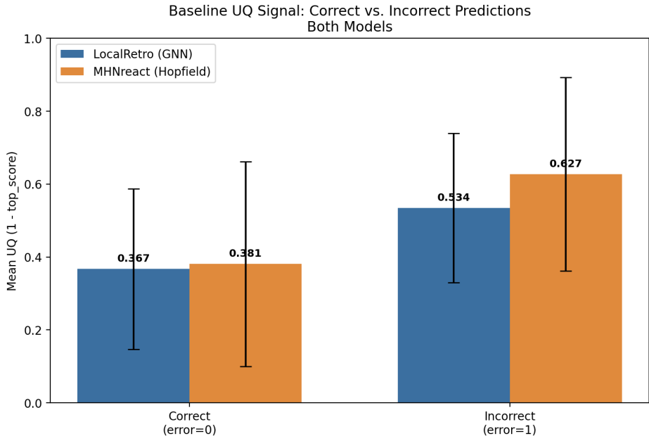
Figure 12: Mean baseline UQ signal ( 1 - \text{top\_score} ), correct vs. incorrect predictions, both models. Error bars show \pm 1 SD. Supports the means reported in Table 1.
