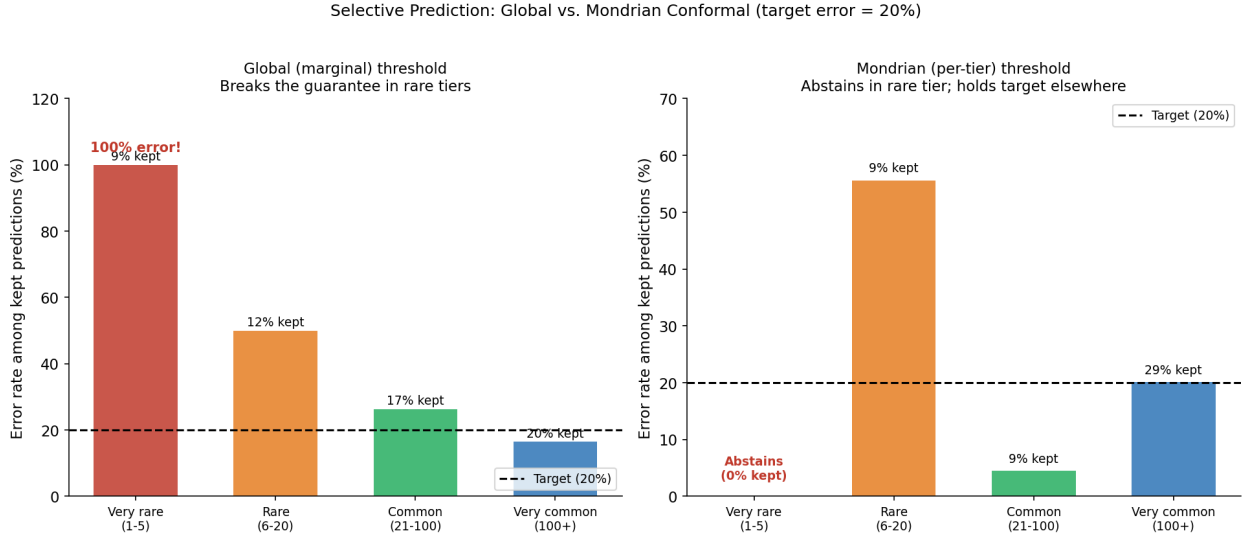
Figure 10: LocalRetro selective prediction under a 20% target error rate. Left : A single global threshold keeps 9% of very-rare predictions with a 100% error rate, far above the target. Right : Mondrian (per-tier) thresholds correctly abstain on the very-rare tier and hold near the target in other tiers. Numbers above bars show the fraction of predictions kept (coverage).
