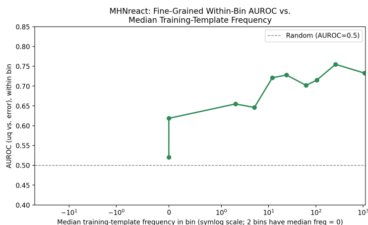
Figure 21: MHNreact: fine-grained within-bin AUROC vs. median training-template frequency. AUROC rises from 0.52 in the zero-frequency bin to a plateau around 0.70–0.75 for established templates, a smoother, more monotonic climb than LocalRetro’s fluctuating 0.64–0.75 range.
