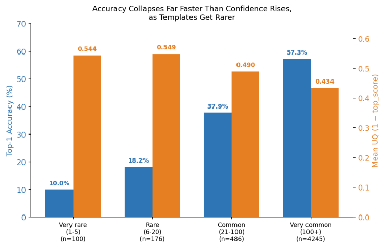
Figure 14: LocalRetro: top 1 accuracy (left axis) and mean UQ (right axis) across four training template frequency tiers. Confidence rises only modestly even as accuracy collapses.
