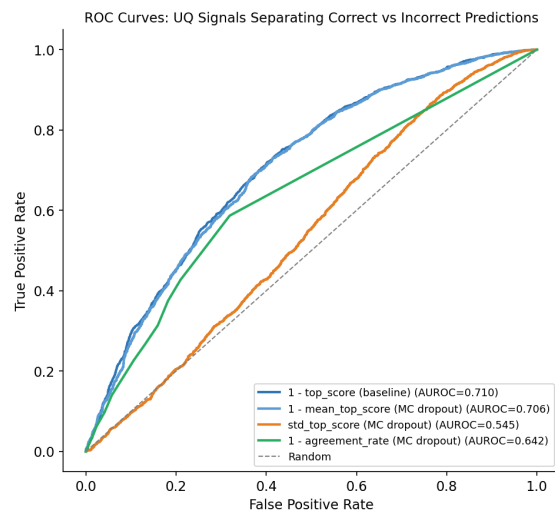
Figure 23: LocalRetro: ROC curves for all evaluated UQ signals.
