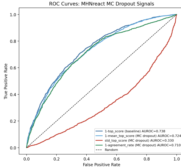
Figure 27: MHNreact: ROC curves for MC dropout signals. The std_top_score curve sits visibly below the diagonal.
