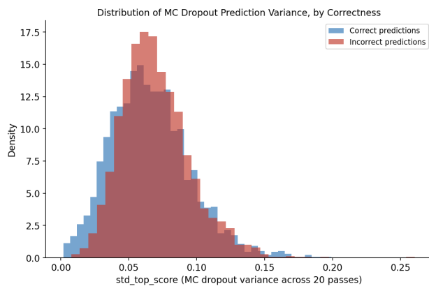
Figure 25: LocalRetro: distribution of MC dropout prediction variance (std_top_score), by correctness.
