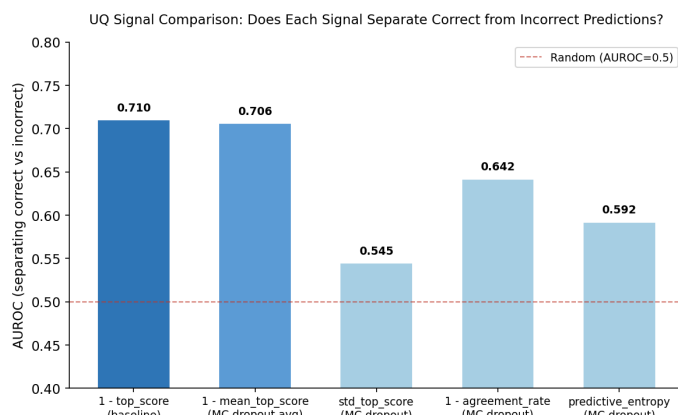
Figure 22: LocalRetro: AUROC of each candidate UQ signal in separating correct from incorrect predictions. Dashed line = random (AUROC = 0.5).
