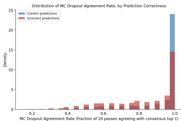
Figure 24: LocalRetro: distribution of MC dropout agreement_rate, by correctness.
