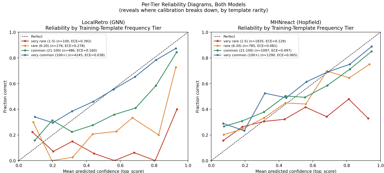
Figure 2: Reliability by training-template frequency tier, both models (side-by-side panels, since each model’s tier boundaries are defined over a different-sized vocabulary: 671 templates for LocalRetro vs. 11,800 for MHNreact, so the tiers are not the same population of reactions and are not meaningfully overlaid on one set of axes). Left (LocalRetro) : tiers fan out sharply: very-common (blue) tracks the diagonal closely while very-rare (red, n=100 ) is noisy and far below it, visually matching the twelve-fold debiased ECE spread (0.024 to 0.291). Right (MHNreact) : tiers stay comparatively clustered together across the whole confidence range, consistent with the uniformly-mildly-miscalibrated signature.
