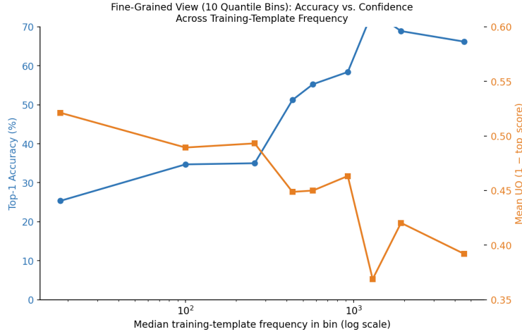
Figure 16: LocalRetro: fine grained (10 quantile bins) accuracy and mean confidence vs. median training template frequency (log x axis).
