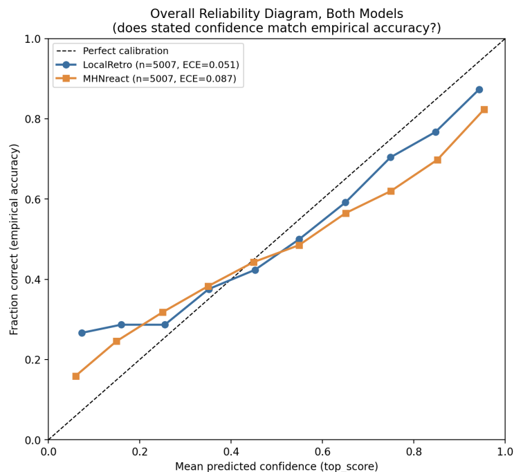
Figure 13: Overall reliability diagram, both models. LocalRetro ( ECE = 0.051 ) is better calibrated on average than MHNreact ( ECE = 0.087 ); both curves sit close to the diagonal in the mid-confidence range and diverge somewhat at the extremes.
