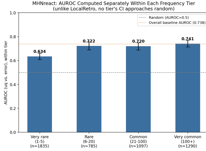
Figure 19: MHNreact: AUROC (uq vs. error) computed separately within each frequency tier, with bootstrap 95% CIs.
