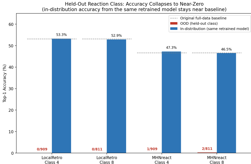
Figure 5: Held-out-class accuracy, all four model/class cells. In-distribution accuracy (blue) tracks each model’s original full-data baseline (dashed line) closely, confirming a healthy retrain. OOD accuracy (red) collapses to 0/909 and 0/811 for LocalRetro, and 1/909 and 2/811 for MHNreact — far below the frequency proxy’s very-rare-tier accuracy (10.0% LocalRetro, 28.4% MHNreact, not shown), confirming genuine distribution shift is a strictly harder regime than the proxy approximated.
