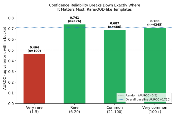
Figure 15: LocalRetro: AUROC (uq vs. error) computed separately within each training frequency tier, with bootstrap 95% CIs.
