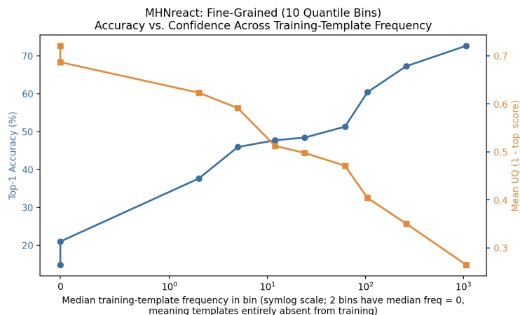
Figure 20: MHNreact: fine-grained (10 quantile bins) accuracy and mean confidence vs. median training-template frequency (symlog x-axis, since 2 bins have median frequency 0).
