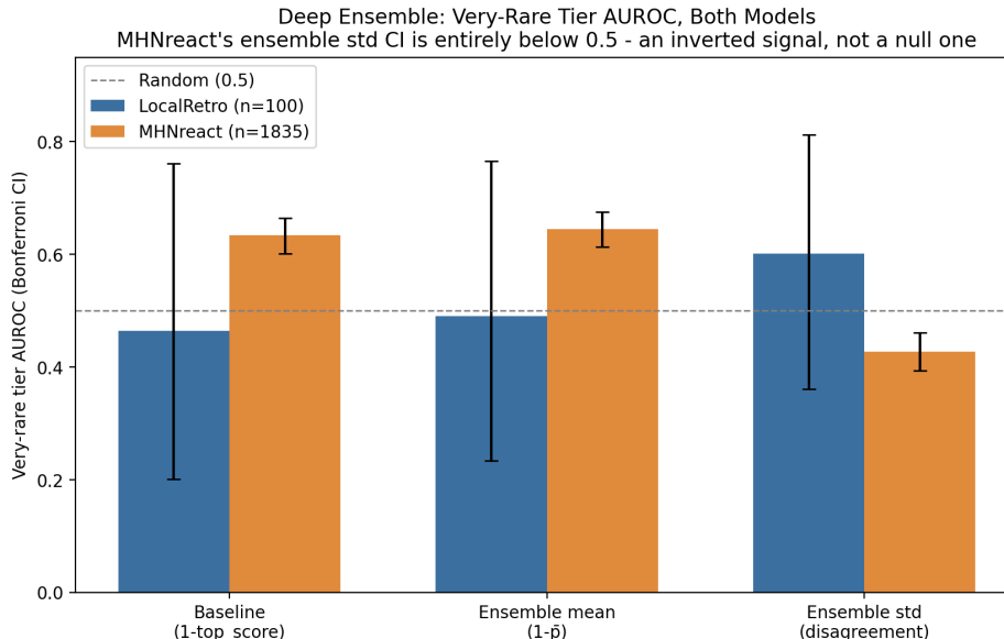
Figure 9: Very-rare tier AUROC with Bonferroni CIs, both models. LocalRetro’s ensemble std CI spans 0.5 (a clean null). MHNreact’s ensemble std CI sits entirely below 0.5, a statistically real inversion, not a wider, less-certain null.
