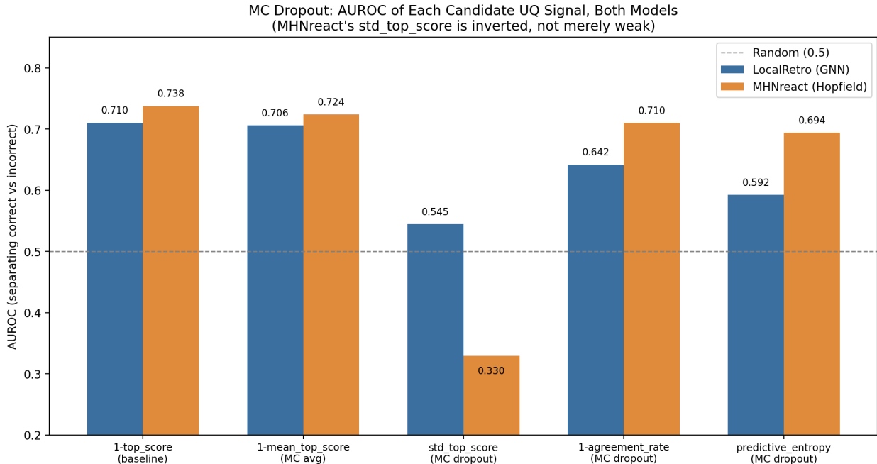
Figure 6: AUROC of each candidate MC dropout signal, both models. MHNreact’s std_top_score is not merely weak like LocalRetro’s; it is inverted, falling well below the random-chance line.
