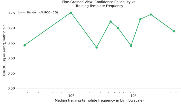
Figure 16: LocalRetro: fine grained within bin AUROC vs. median training template frequency. Reliability stays broadly stable (0.64 to 0.75) outside the most extreme rarity tail.
