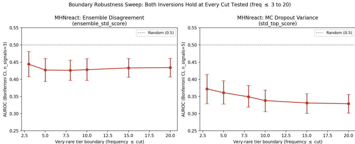
Figure 7: Boundary robustness sweep for both MHNreact inversion claims: AUROC and Bonferroni-corrected CI recomputed at six different very-rare-tier boundary definitions ( \text{freq} \leq 3, 5, 8, 10, 15, 20 ). Both inversions (MC dropout variance, right; ensemble disagreement, left) hold at every cut tested: the CI excludes 0.5 in all six cases for both signals. A claim that holds only at one arbitrary boundary would be fragile; this one does not.
