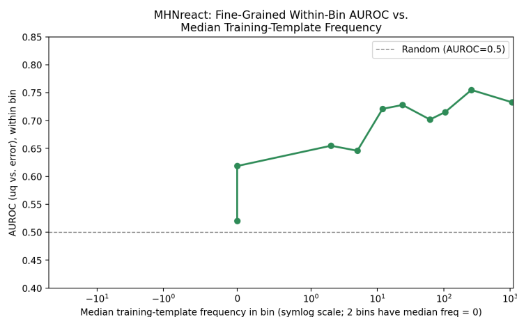
Figure 20: MHNreact: fine-grained within-bin AUROC vs. median training-template frequency. AUROC rises from 0.52 in the zero-frequency bin to a plateau around 0.70–0.75 for established templates, a smoother, more monotonic climb than LocalRetro’s fluctuating 0.64–0.75 range.
