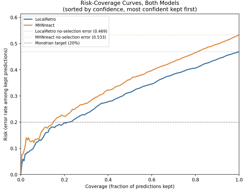
Figure 29: Overall risk-coverage curves, both models (sorted by confidence, most-confident-first, no tier stratification).
