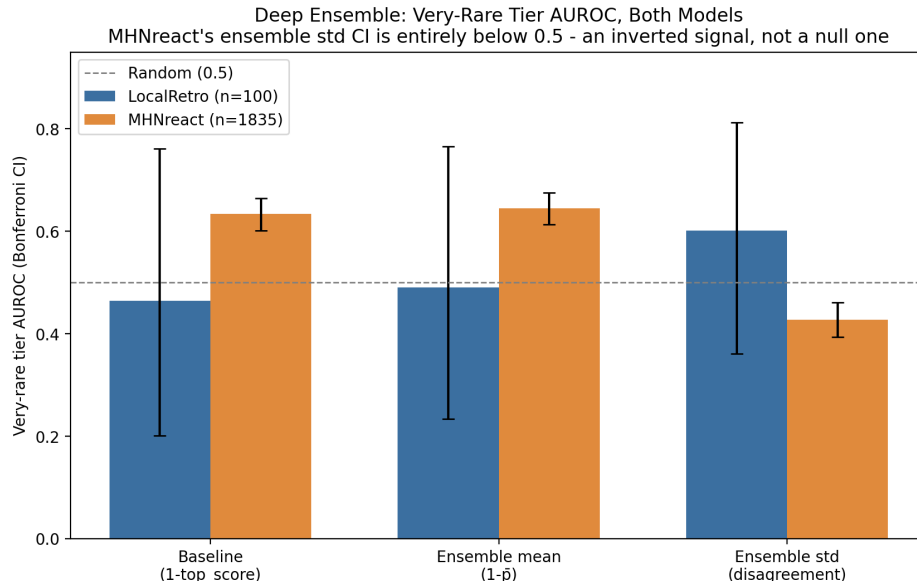
Figure 8: Very-rare tier AUROC with Bonferroni CIs, both models. LocalRetro’s ensemble std CI spans 0.5 (a clean null). MHNreact’s ensemble std CI sits entirely below 0.5, a statistically real inversion, not a wider, less-certain null.
