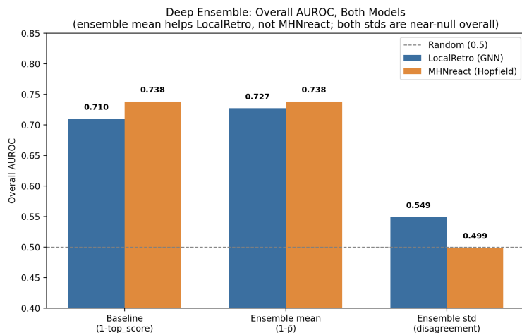
Figure 27: Deep ensemble overall (non-tiered) AUROC, both models. Ensemble mean helps LocalRetro but not MHNreact; both ensemble-std signals hover near random overall, which is why the very-rare-tier breakdown (main text Figure 8) is the figure that carries the argument.
