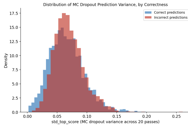
Figure 24: LocalRetro: distribution of MC dropout prediction variance (std_top_score), by correctness.
