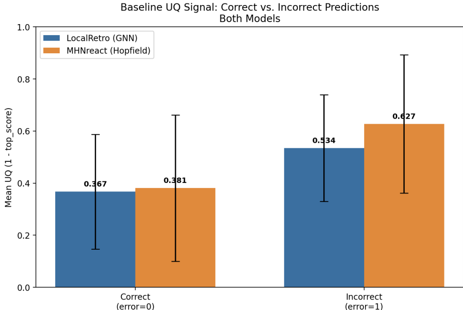
Figure 11: Mean baseline UQ signal ( 1 - \text{top\_score} ), correct vs. incorrect predictions, both models. Error bars show \pm 1 SD. Supports the means reported in Table 1.
