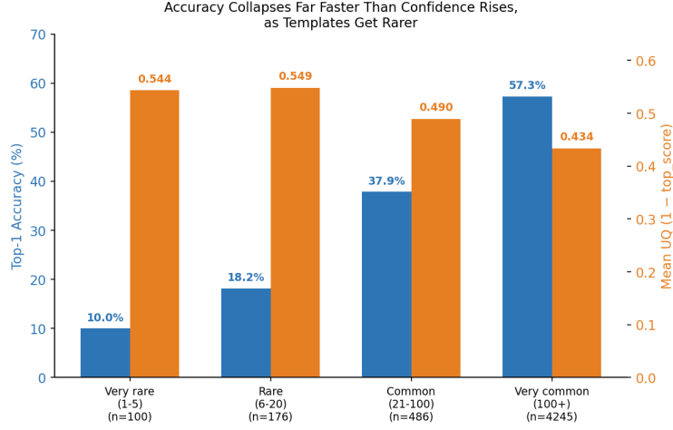
Figure 13: LocalRetro: top 1 accuracy (left axis) and mean UQ (right axis) across four training template frequency tiers. Confidence rises only modestly even as accuracy collapses.
