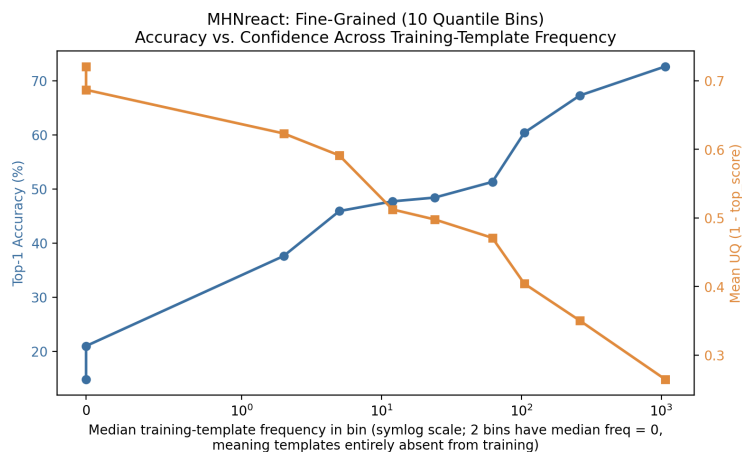
Figure 19: MHNreact: fine-grained (10 quantile bins) accuracy and mean confidence vs. median training-template frequency (symlog x-axis, since 2 bins have median frequency 0).
