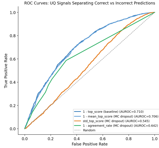
Figure 22: LocalRetro: ROC curves for all evaluated UQ signals.
