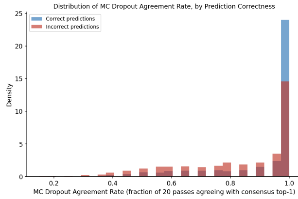
Figure 23: LocalRetro: distribution of MC dropout agreement_rate, by correctness.
