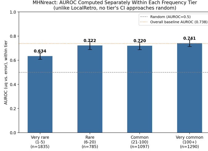
Figure 18: MHNreact: AUROC (uq vs. error) computed separately within each frequency tier, with bootstrap 95% CIs.
