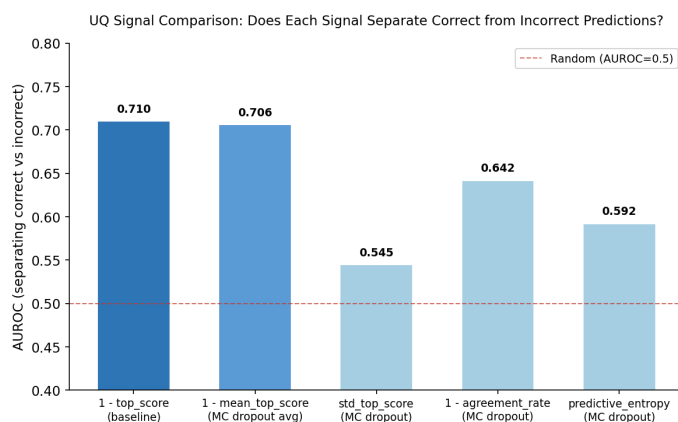
Figure 21: LocalRetro: AUROC of each candidate UQ signal in separating correct from incorrect predictions. Dashed line = random (AUROC = 0.5).
