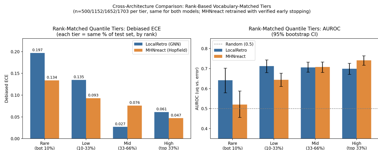
Figure 3: Rank-based vocabulary-matched tier comparison. Left : Debiased ECE by tier. Both models have highest ECE in the rare tier, but their profiles differ: LocalRetro shows a sharp drop from rare to mid (0.197 to 0.027), while MHNreact declines smoothly and monotonically (0.134 to 0.047). Right : AUROC by tier with 95% bootstrap CIs; both models maintain discrimination above random across all tiers.
