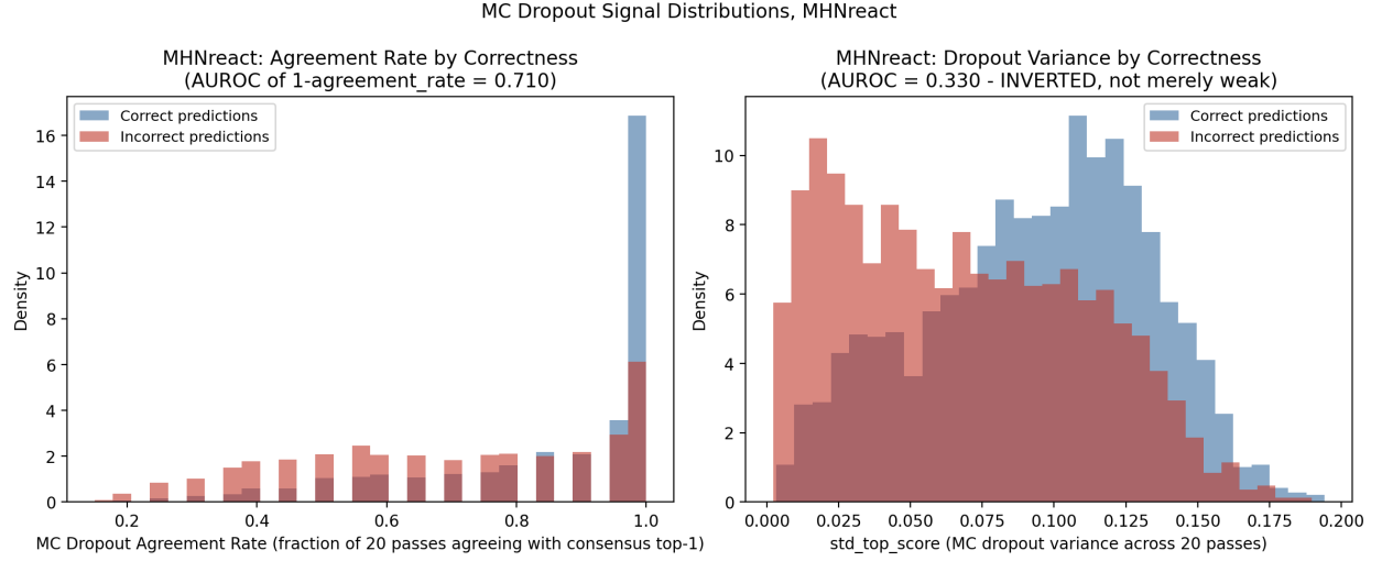
Figure 25: MHNreact: MC dropout signal distributions by correctness. Left : agreement rate. Right : dropout variance, showing the inversion visually.
