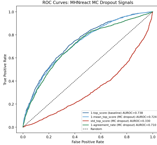
Figure 26: MHNreact: ROC curves for MC dropout signals. The std_top_score curve sits visibly below the diagonal.
