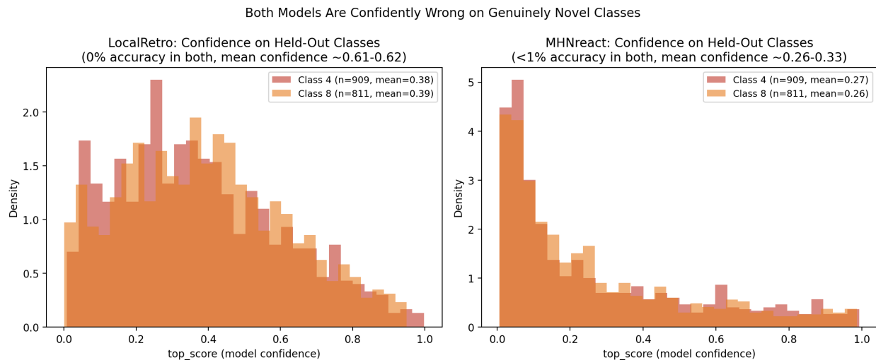
Figure 5: Confidence distribution on the held-out (OOD) test sets, both models. Despite 0% (LocalRetro) or near-0% (MHNreact) actual accuracy, mean confidence stays well above zero in every case (LocalRetro: 0.376–0.390; MHNreact: 0.259–0.269) — both models remain confidently wrong on genuinely novel reaction classes rather than correctly signaling low confidence, the calibration failure mode most relevant to deployment.
