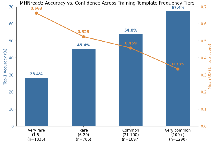
Figure 17: MHNreact: top-1 accuracy (left axis) and mean UQ (right axis) across four training-template frequency tiers. Accuracy rises from 28.4% to 67.4%, a 39-point spread, versus LocalRetro’s 47.3-point collapse from a much smaller very-rare base rate.
