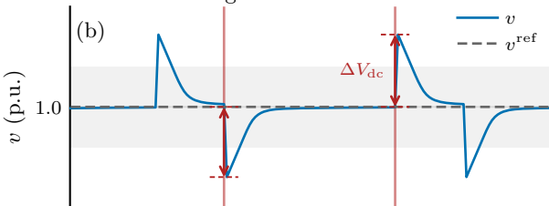
Voltage with fixed-reference
