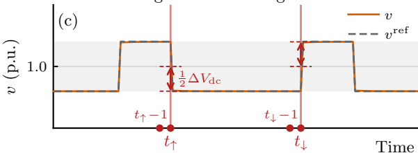
Voltage with switching-reference
