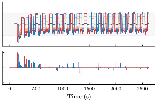
Switching-reference
