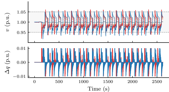
Fixed-reference
