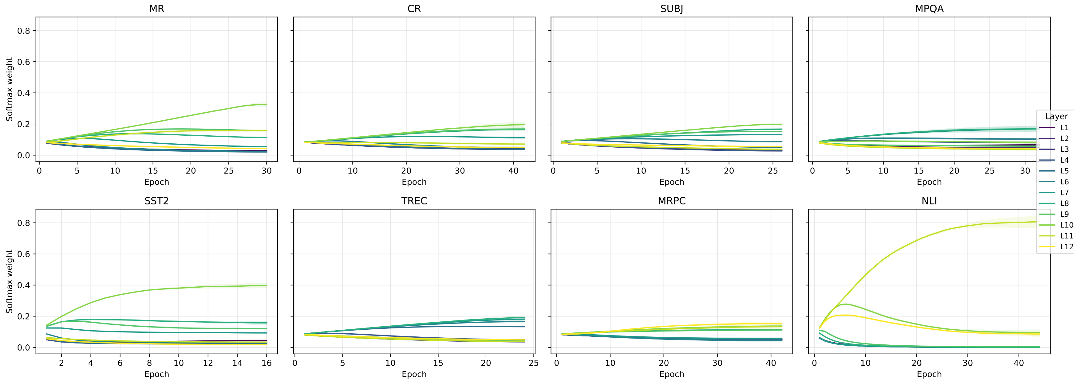
Layer weight evolution during training (mean \pm std over seeds)
