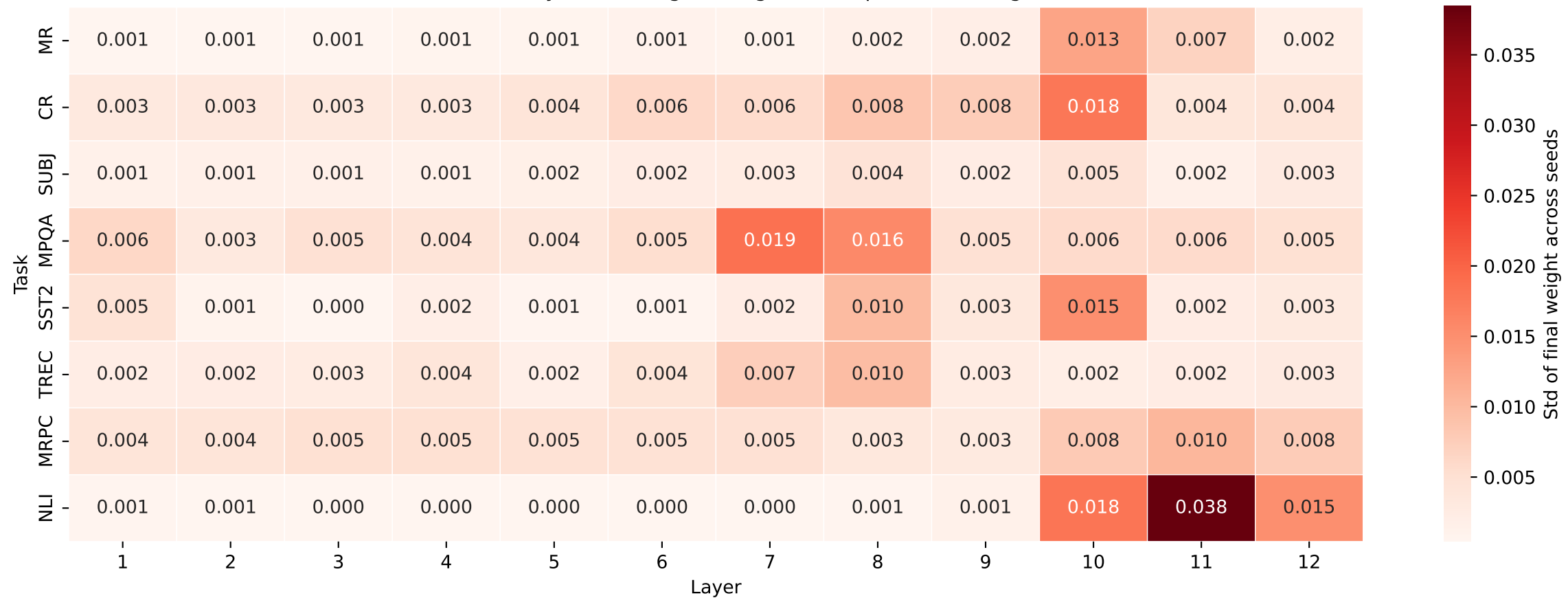
Cross-seed stability of converged weights (complement to Figure 9)
