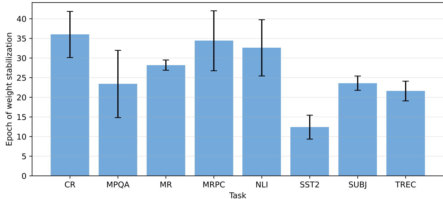
Time to weight stabilization (tol = 1e-3, mean \pm std over seeds)
