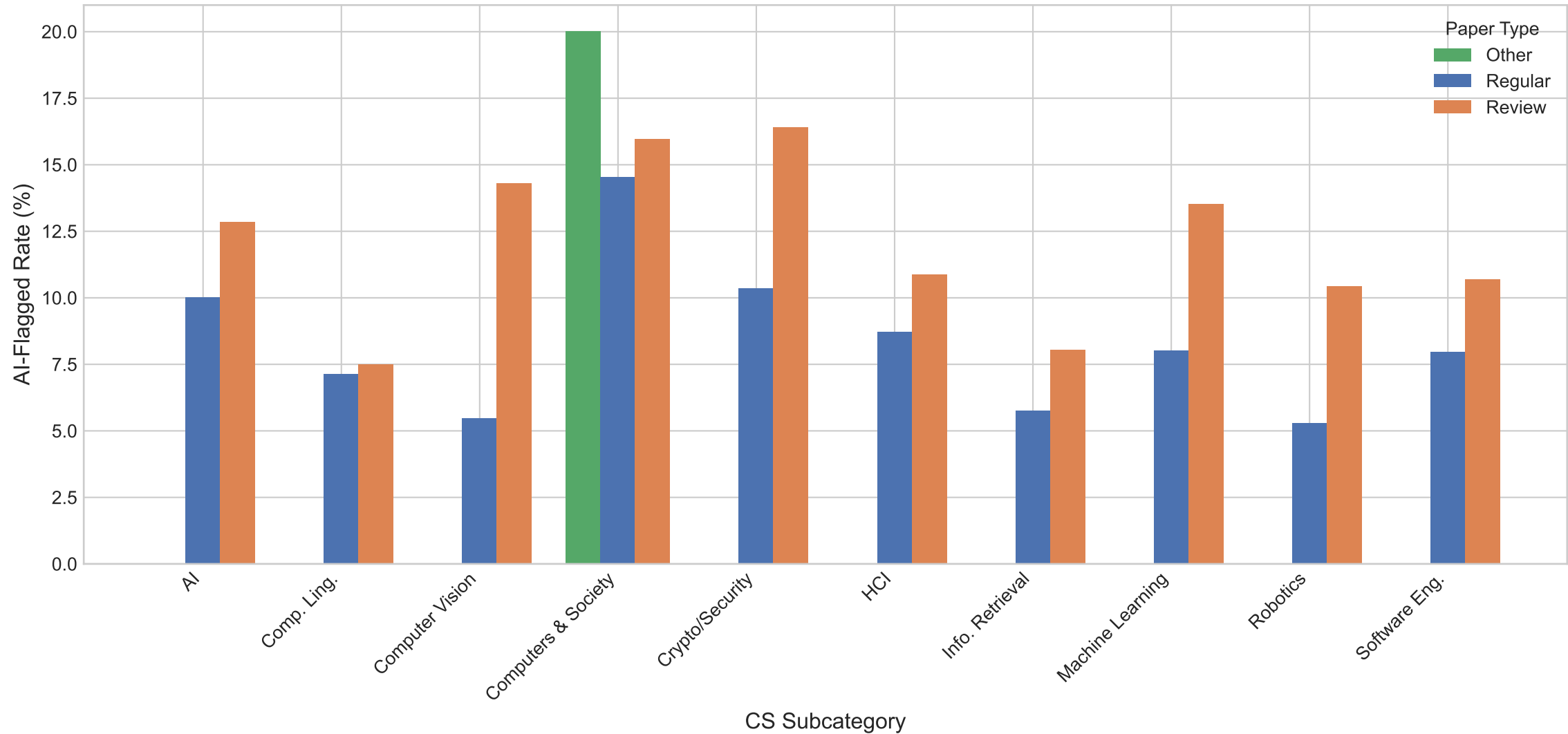
AI Detection Rate by Paper Type and Subcategory
