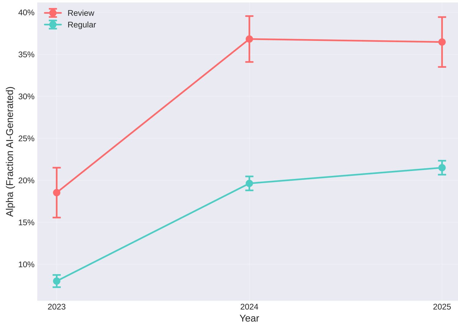
Alpha Estimates by Year (Post-LLM)
