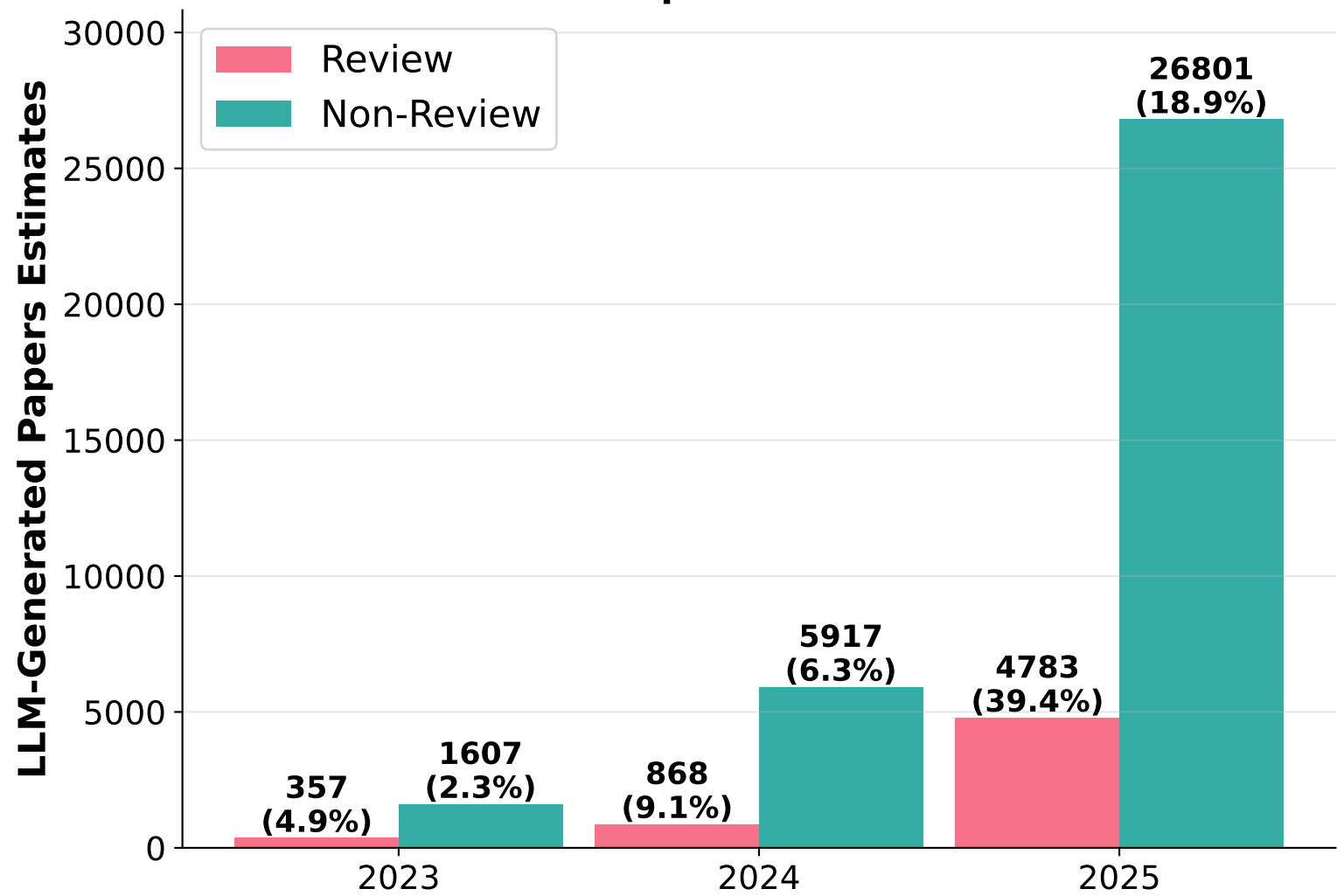
Computer Science
