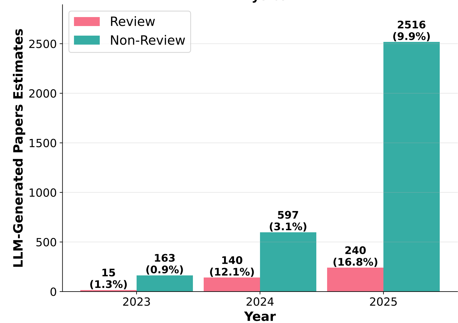
Physics
