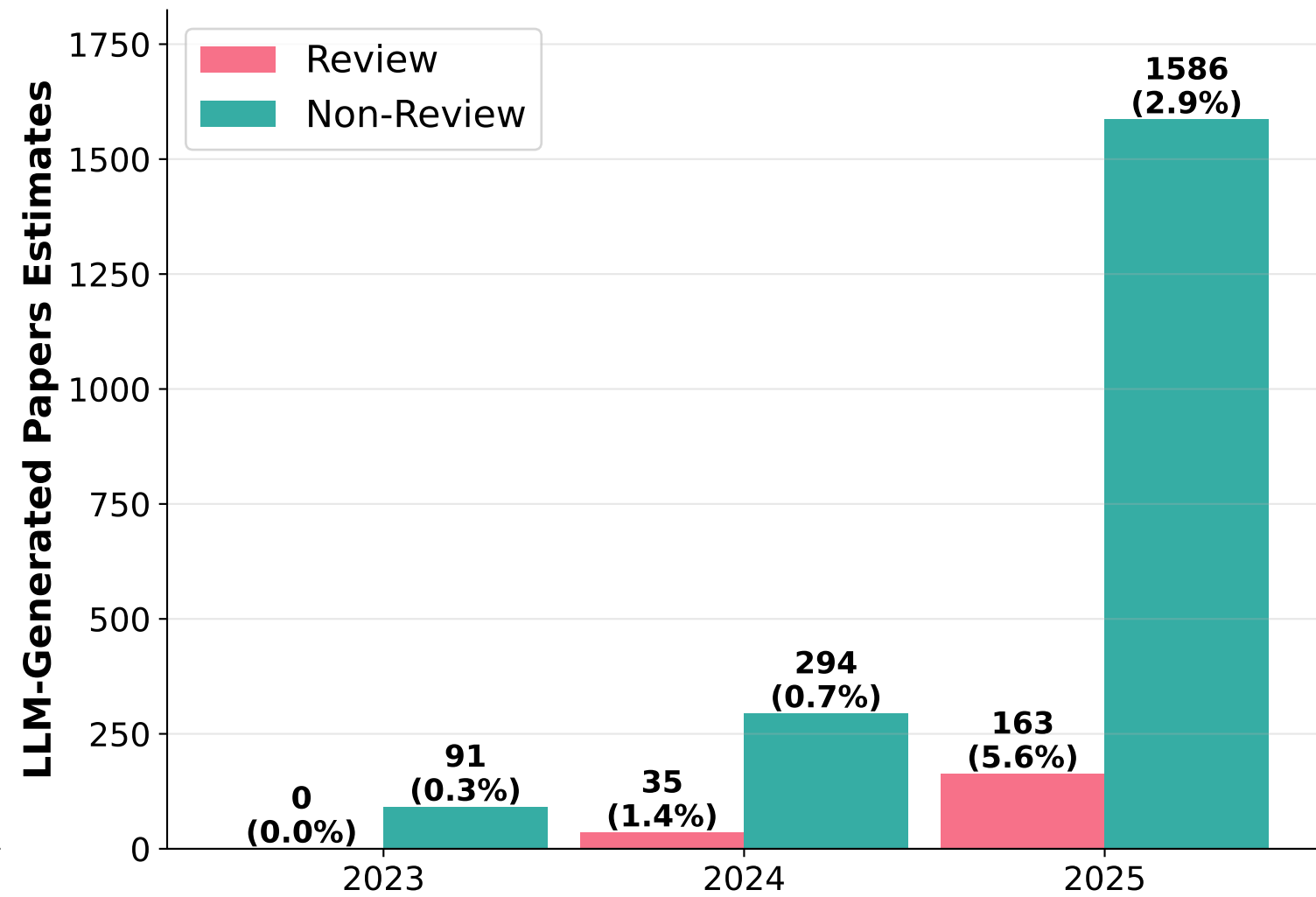
Mathematics
