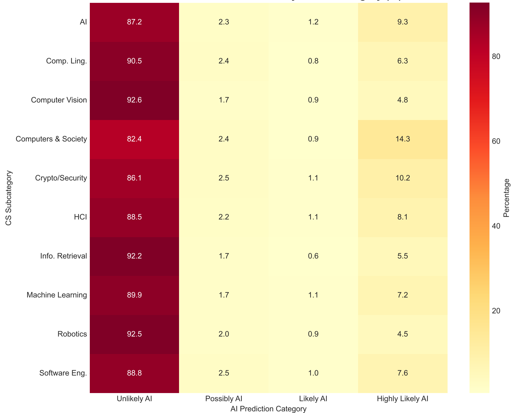
Distribution of AI Predictions by CS Subcategory (%)
