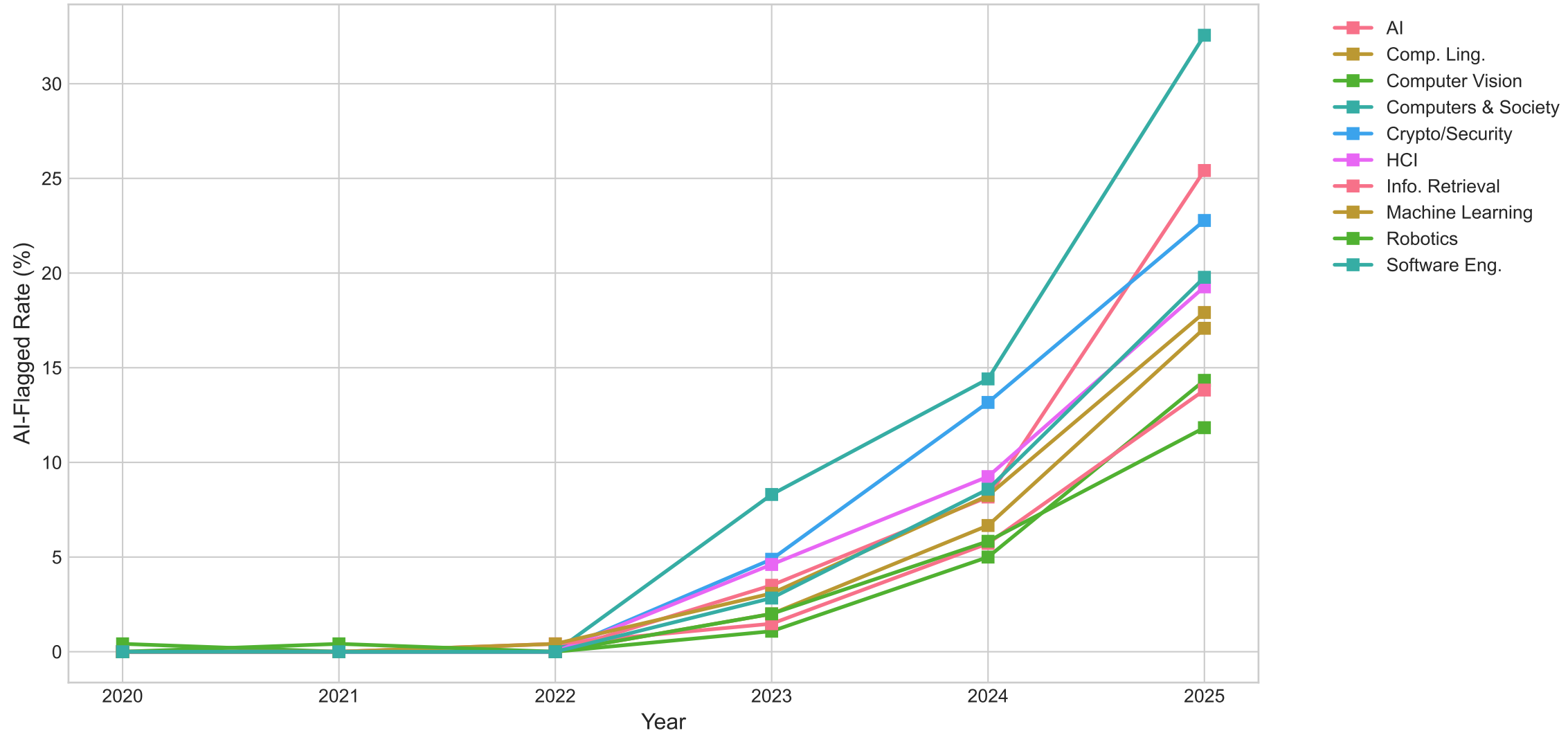
AI Detection Rates by Year and CS Subcategory
