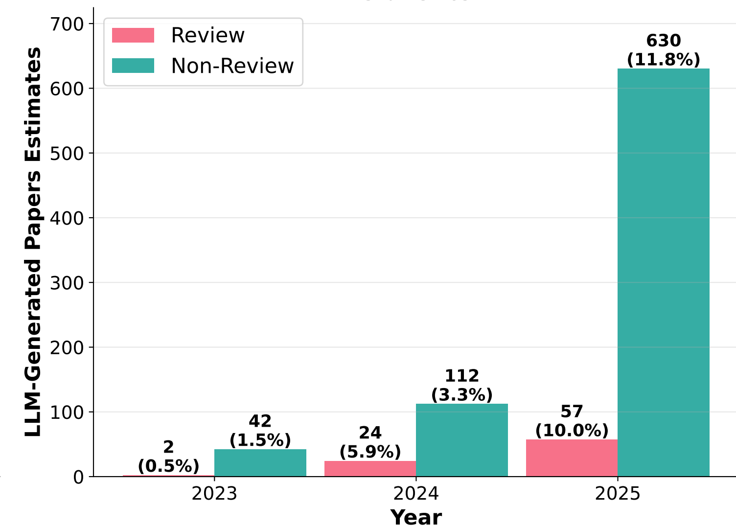
Statistics
