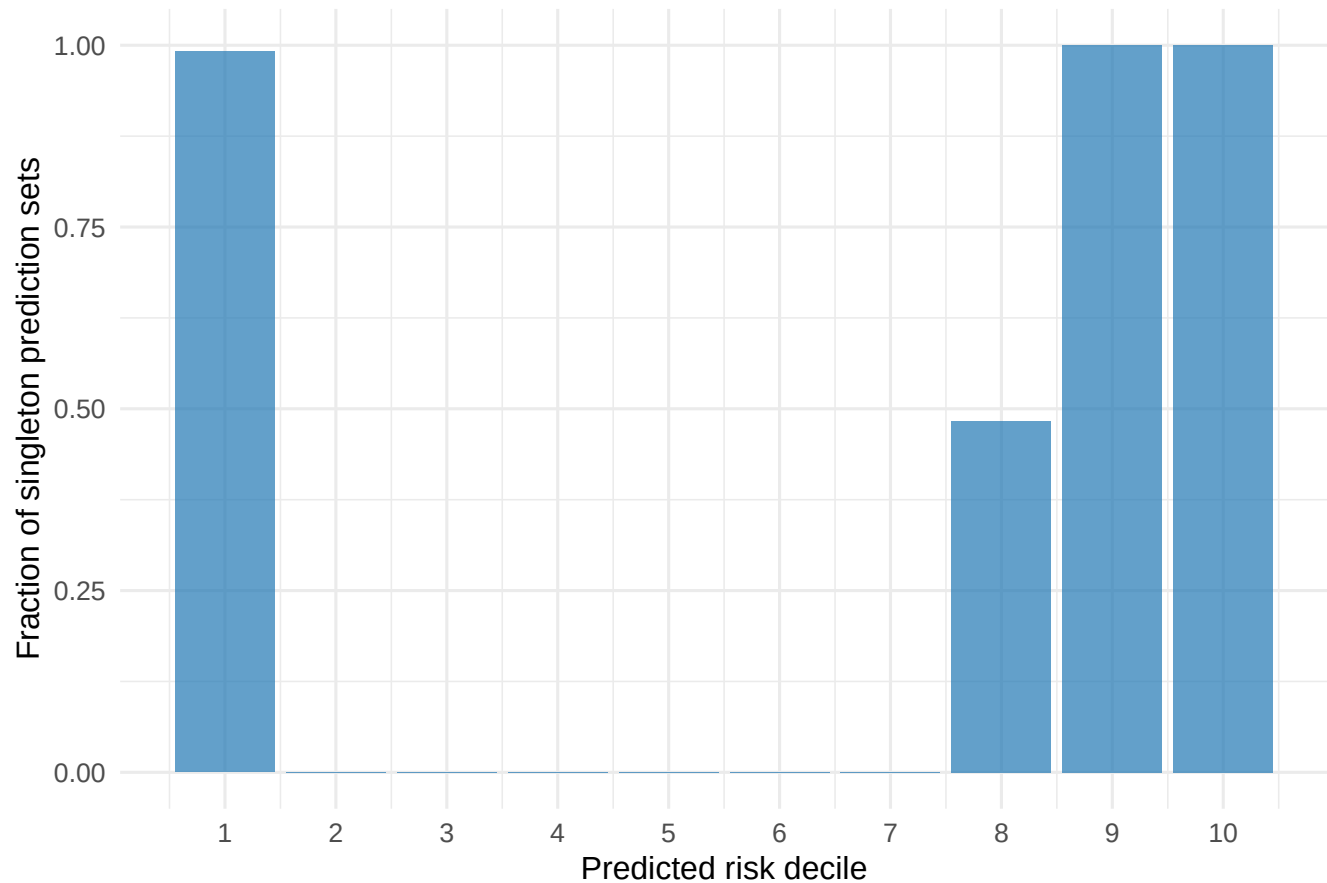
Figure 5: Conformal Informativeness by Risk Decile
