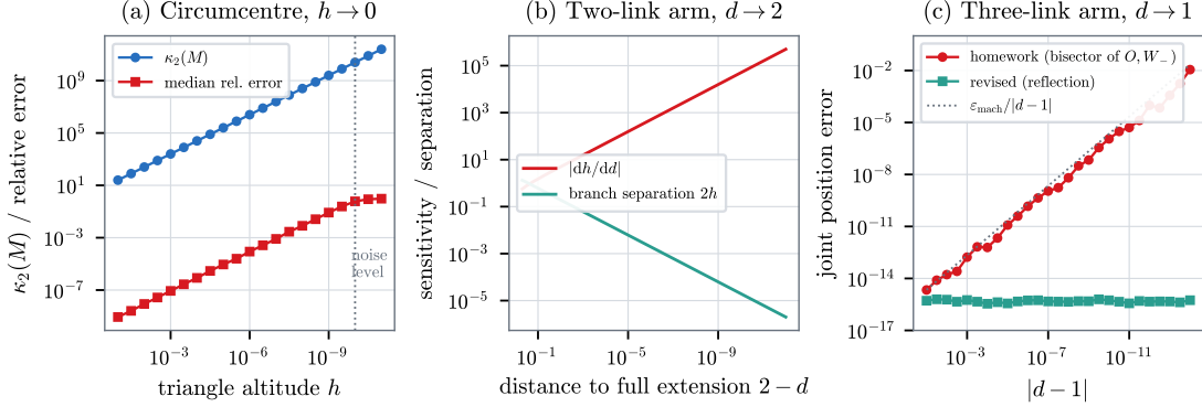
Figure 5: Three limits. (a) Geometric singularity: the circumcentre becomes sensitive as the triangle approaches collinearity. (b) Geometric singularity: the elbow branches merge at full extension while the derivative of their height diverges. (c) Representation singularity: the original three-link construction loses accuracy like \varepsilon_{\text{mach}}/|d-1| near d = 1 , where the arm is regular; the reflection-based construction does not.
