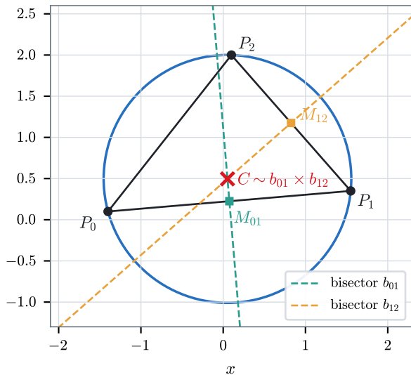
(a) Circumcentre as a projective meet
