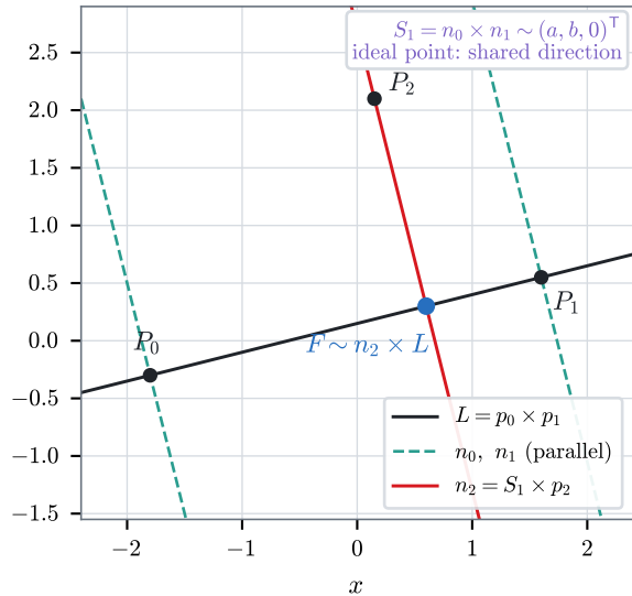
(b) A finite foot through an ideal point
