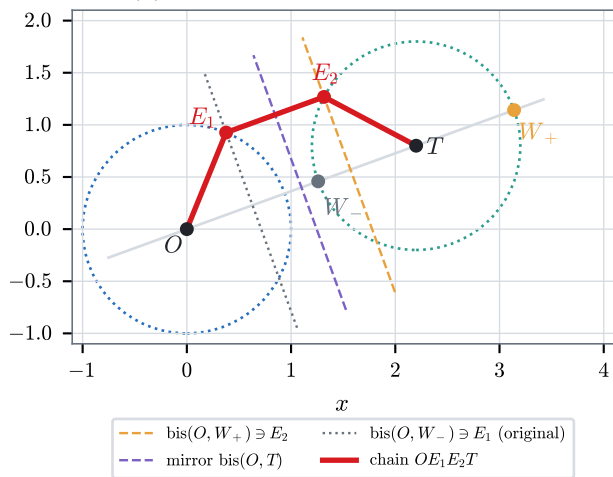
(b) Three-link arm: isosceles trapezoid
