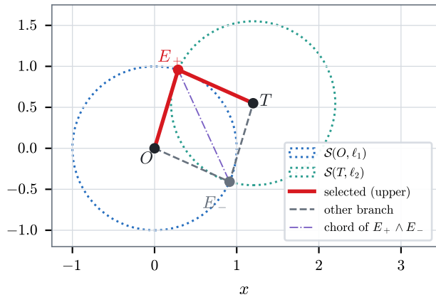
(a) Two-link arm: circle-circle meet
