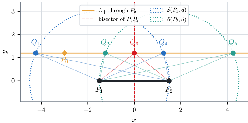
(a) Five apices as line-locus intersections
