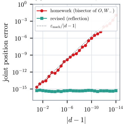
(c) Three-link arm, d \rightarrow 1
