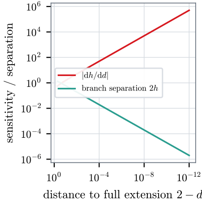
(b) Two-link arm, d \rightarrow 2
