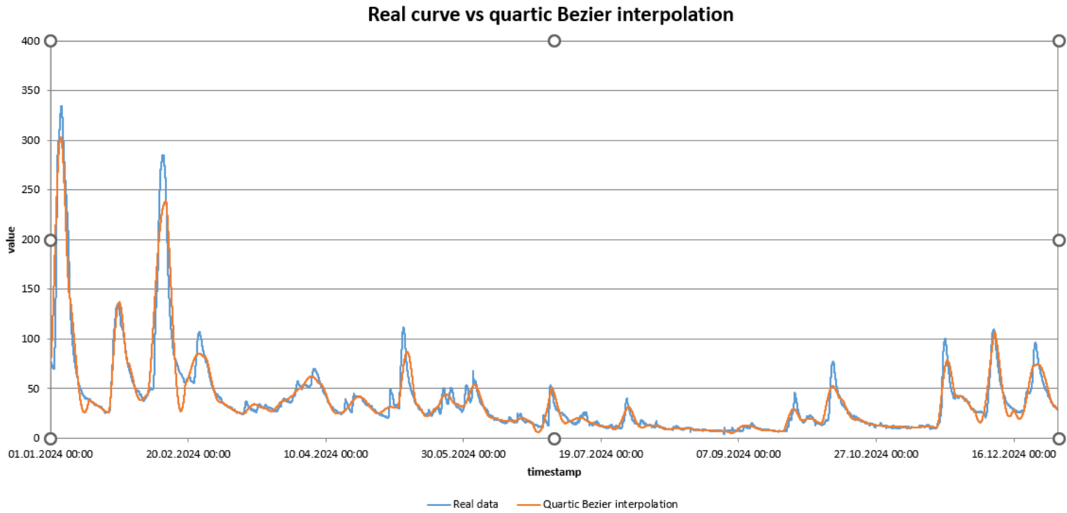
Figure 3: Interpolated curve compared with measured data.
