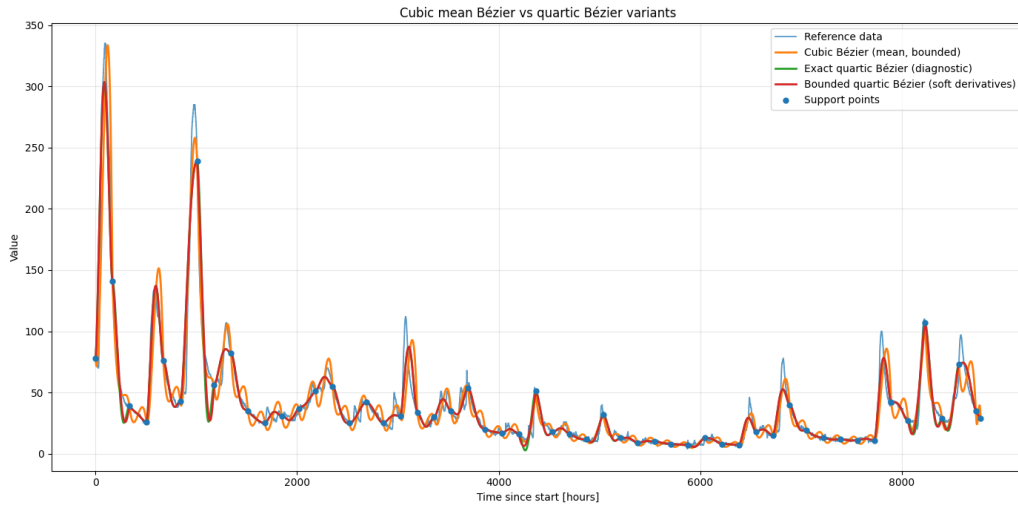
Figure 4: Comparison of the reference data, support points, and the three Bézier interpolation methods.
