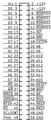
PC-8001 BUS J2
