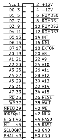
PC-8001 BUS J1
