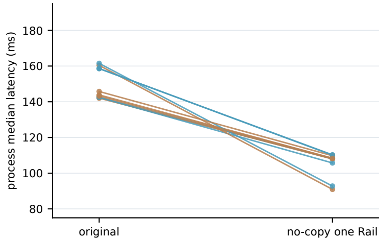
A. Same object/HCA, paired processes
