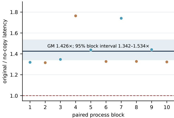
B. All ten blocks favor no-copy
