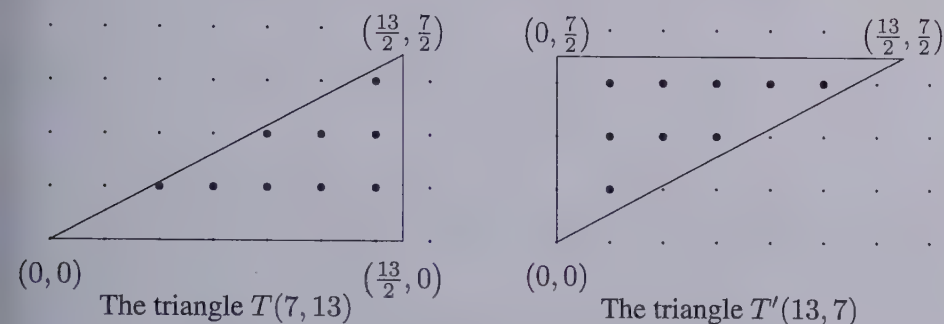
Figure 23.2: Counting Integer Points in Triangles
