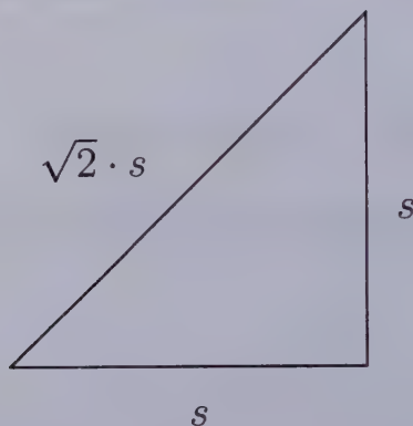
Figure 37.1: An Incommensurable Hypotenuse
