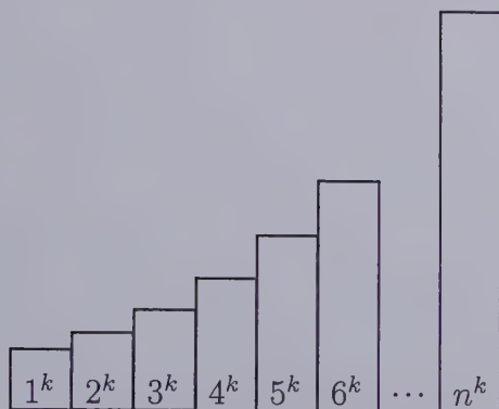
Figure 40.1: Rectangles Whose Total Area Is 1^k + 2^k + \cdots + n^k
