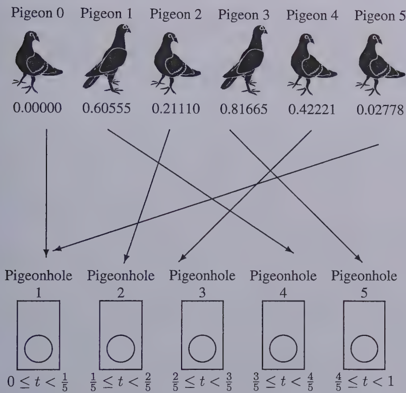
Figure 33.1: Pigeons and Pigeonholes for D = 13 and Y = 5
