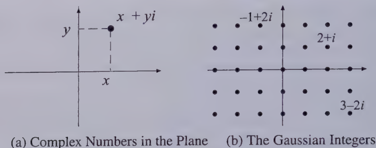
Figure 35.1: The Geometry of the Complex Numbers
