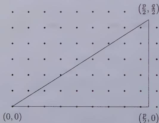
Figure 23.1: The Triangle T(q, p)
