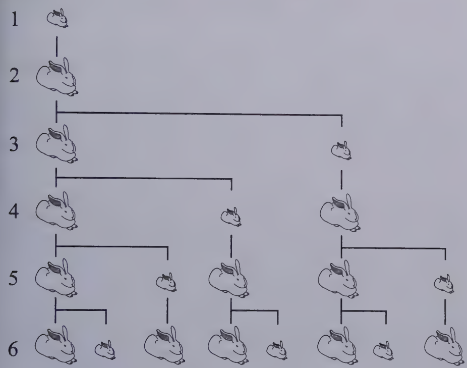
Figure 39.1: Fibonacci's Rabbits (each rabbit image represents a pair)
