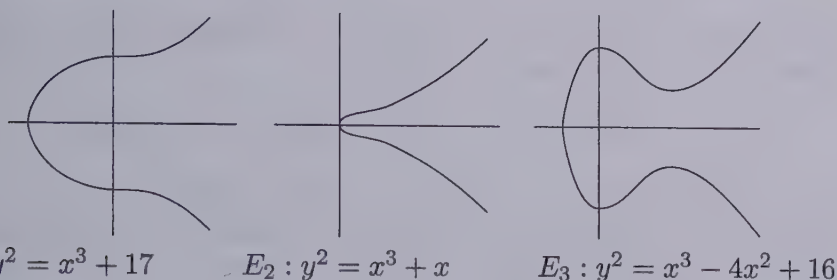
Figure 41.1: Graphs of Three Representative Elliptic Curves
