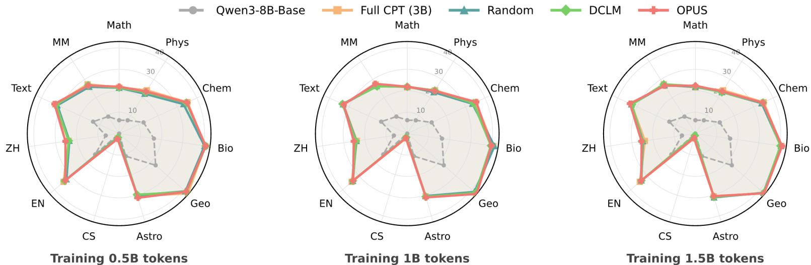
(a) OlympicArena
