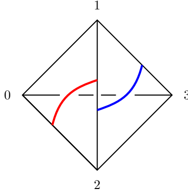
FIGURE 4. The fundamental domain in T_0 for the action of \mathfrak{Set} . The vertices are barycenters of a vertex, edge, face, and of T_0 , and are labeled here by 0, 1, 2, and 3, respectively.
