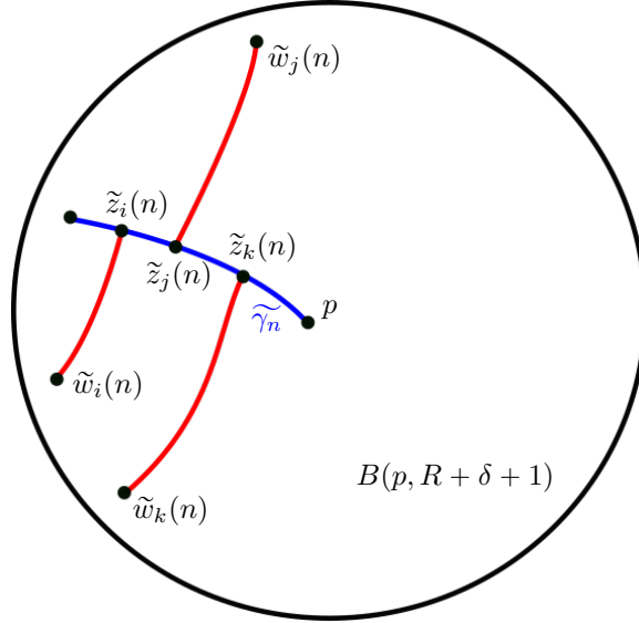
FIGURE 9. The points \{\tilde{w}_0(n), \tilde{w}_1(n), \dots, \tilde{w}_{n-1}(n)\} are all contained in the ball B(p, R + \delta + 1) \subset \mathbb{H}^3 .
