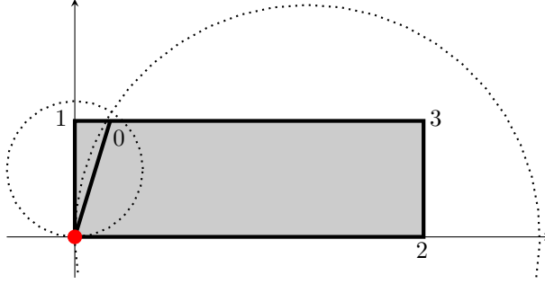
FIGURE 6. View of P \subset \mathbb{H}^3 from above with red vertex and numbers matching those from Figures 4 and 5. The blue vertex is at infinity.
