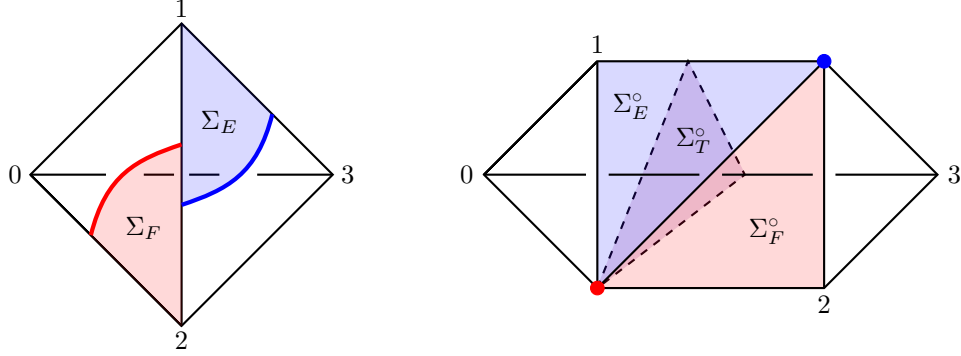
FIGURE 8. Left: Pieces of \Sigma_E and \Sigma_F in P , the fundamental polyhedron for the action of \mathfrak{T}et . Right: The totally geodesic representatives of \Sigma_E^\circ , \Sigma_F^\circ , and \Sigma_T^\circ are constructed by gluing together the indicated totally geodesic polygons in P .
