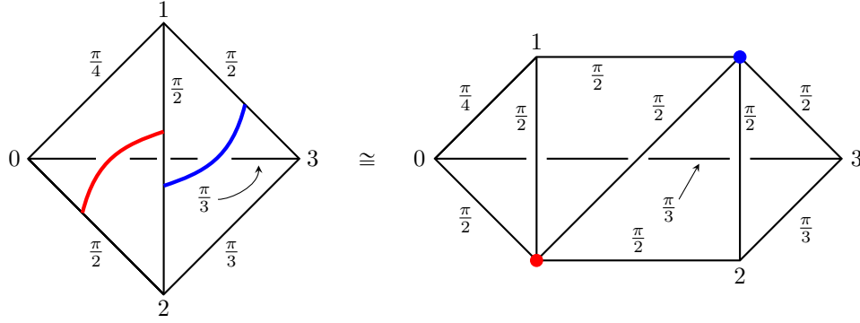
FIGURE 5. Left: Dihedral angles for hyperbolic structure on \Delta \setminus L_0 . Right: Partially ideal polyhedron P with ideal vertices obtained by collapsing arcs to a point (illustrated by a dot). Vertex numbers and labels match Figure 4.
