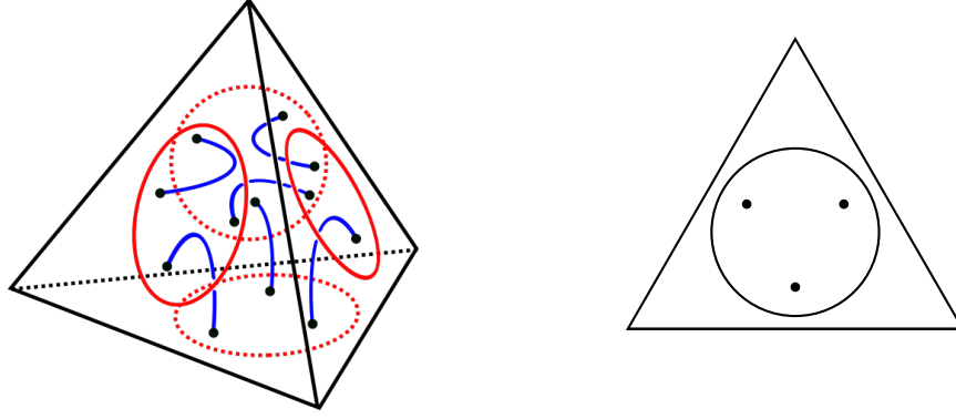
FIGURE 3. Left: The tangle L_0 \subset T_0 . Right: The intersection of L_0 with the face.
