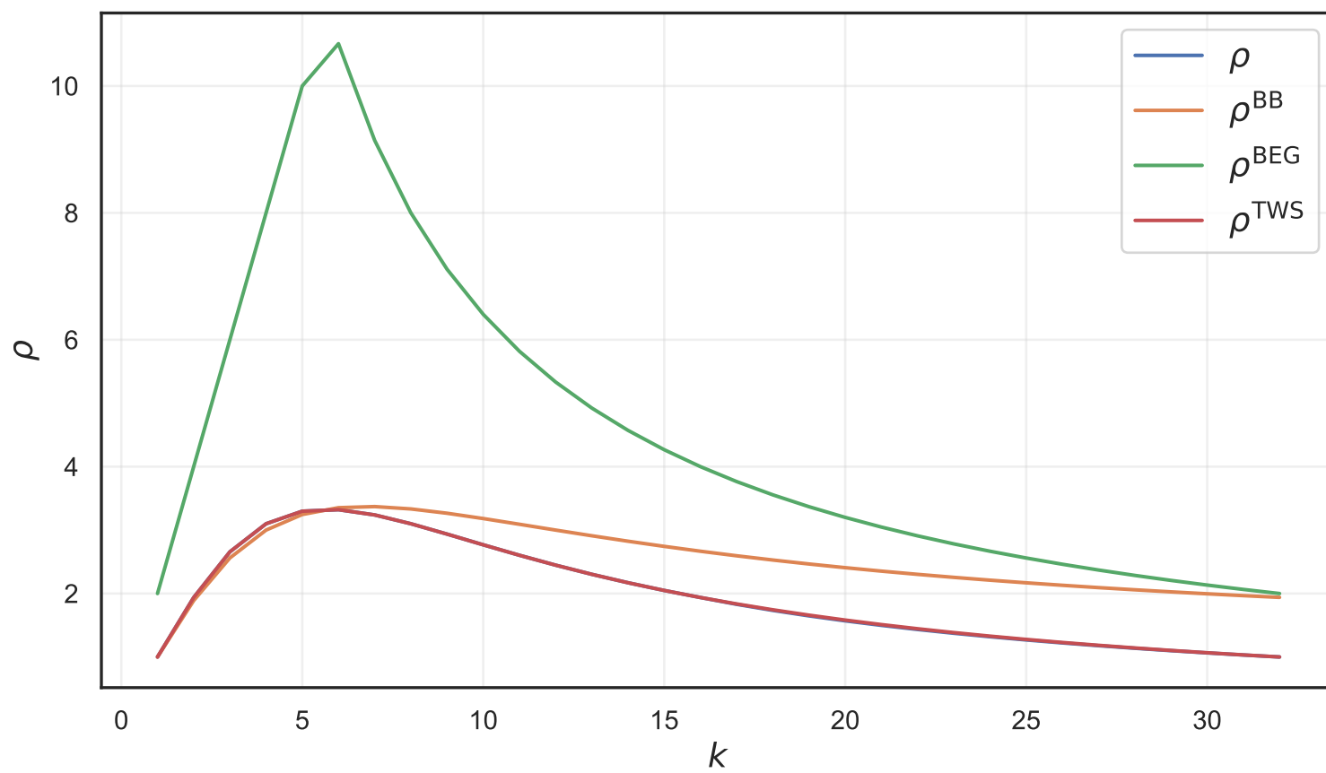
m = 32
