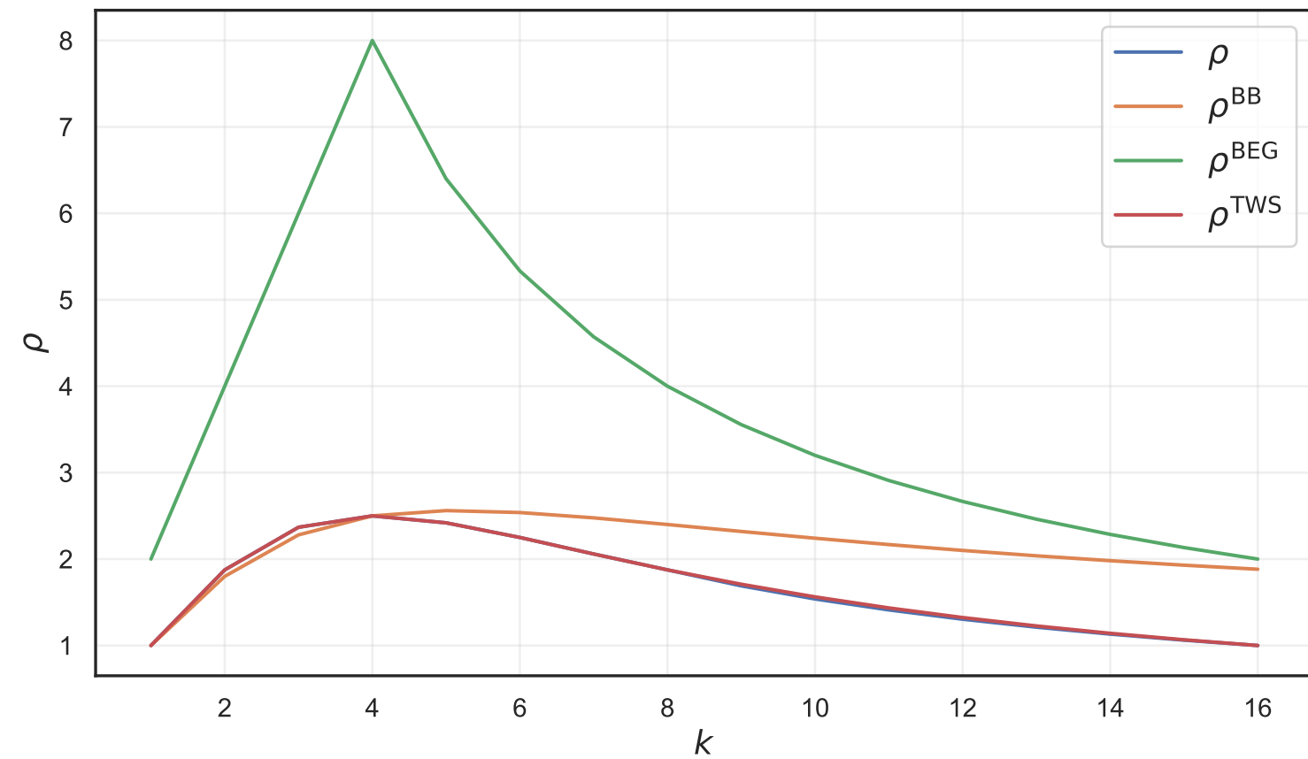
m = 64
