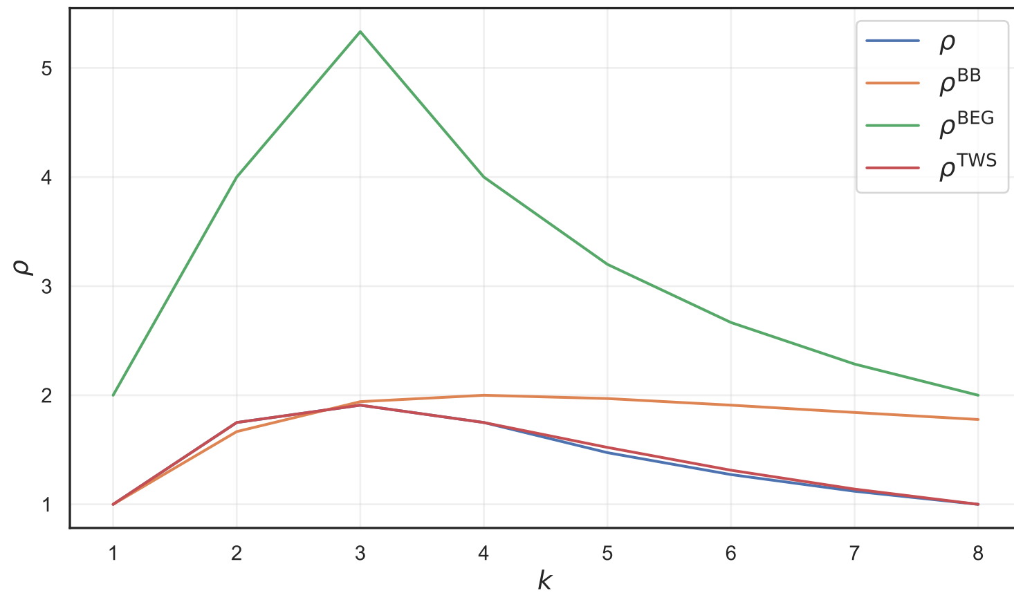
m = 32
