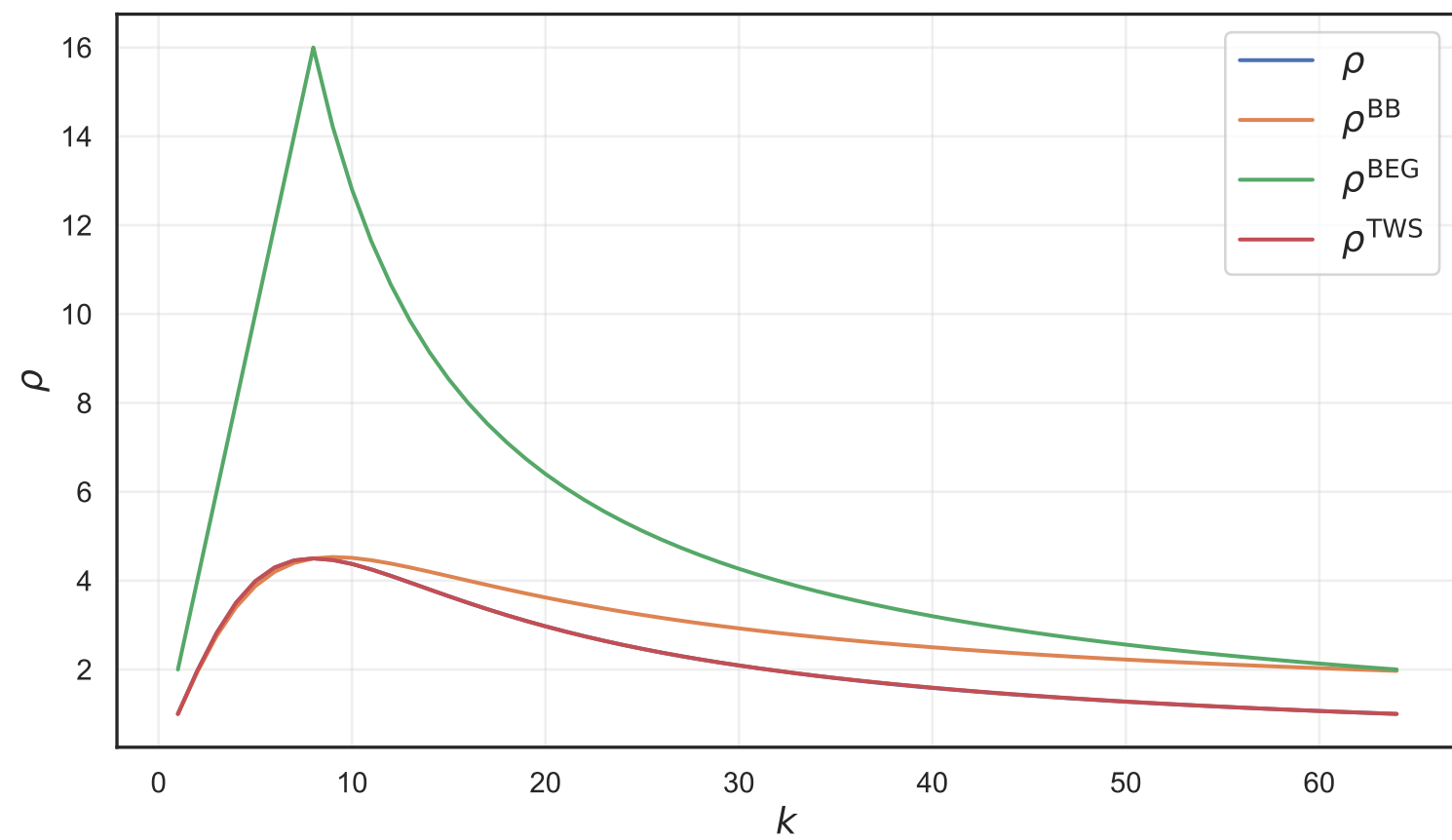
m = 64
