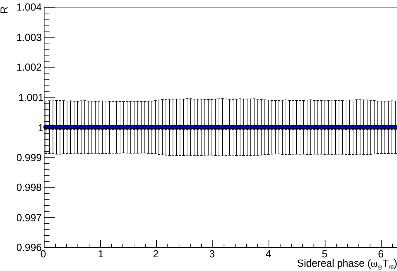
Fit to toy 36, signal shape: d0
