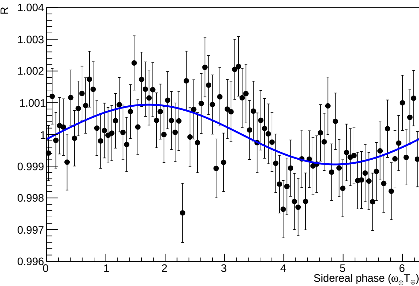
Fit to toy 39, signal shape: d0
