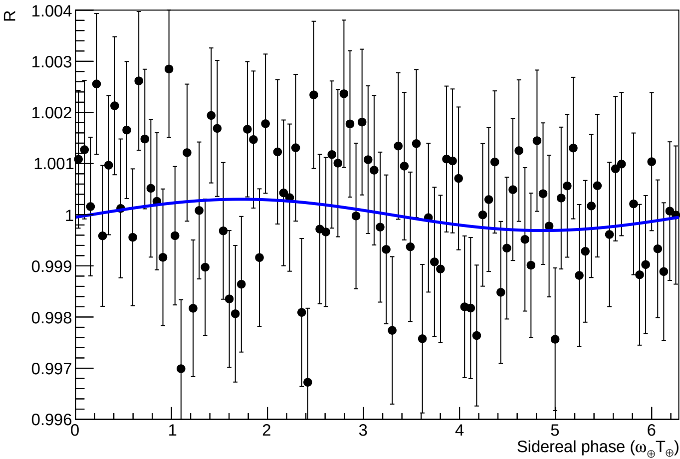
Fit to toy 11, signal shape: d0
