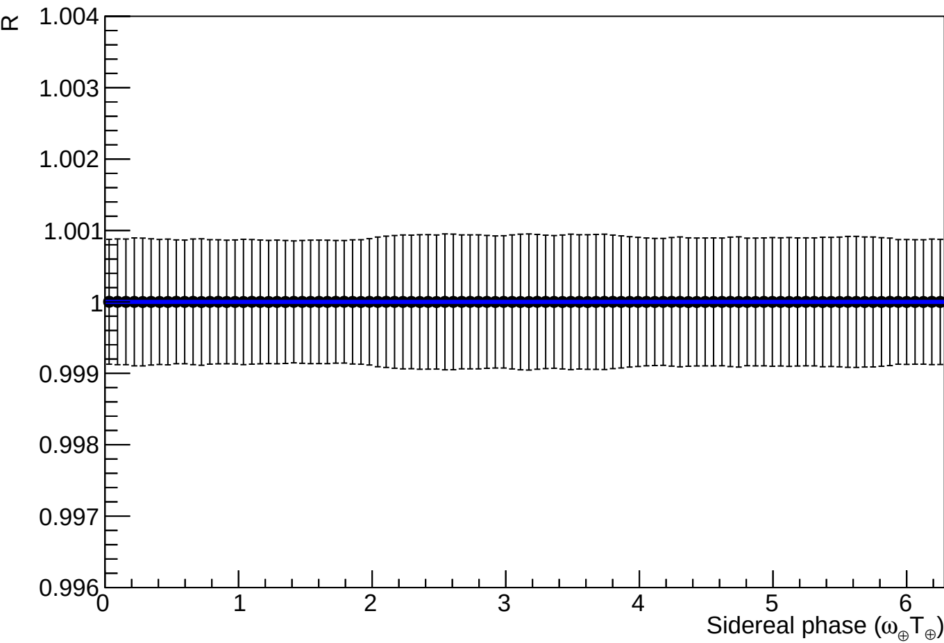
Fit to toy 36, signal shape: d1
