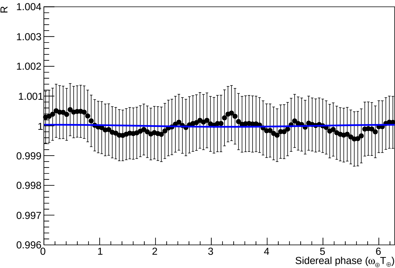
Fit to toy 38, signal shape: d1
