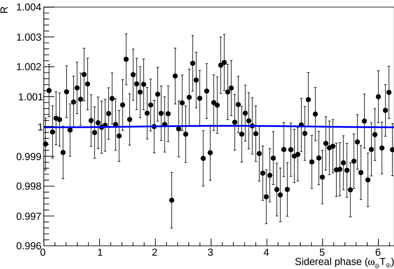
Fit to toy 39, signal shape: d1
