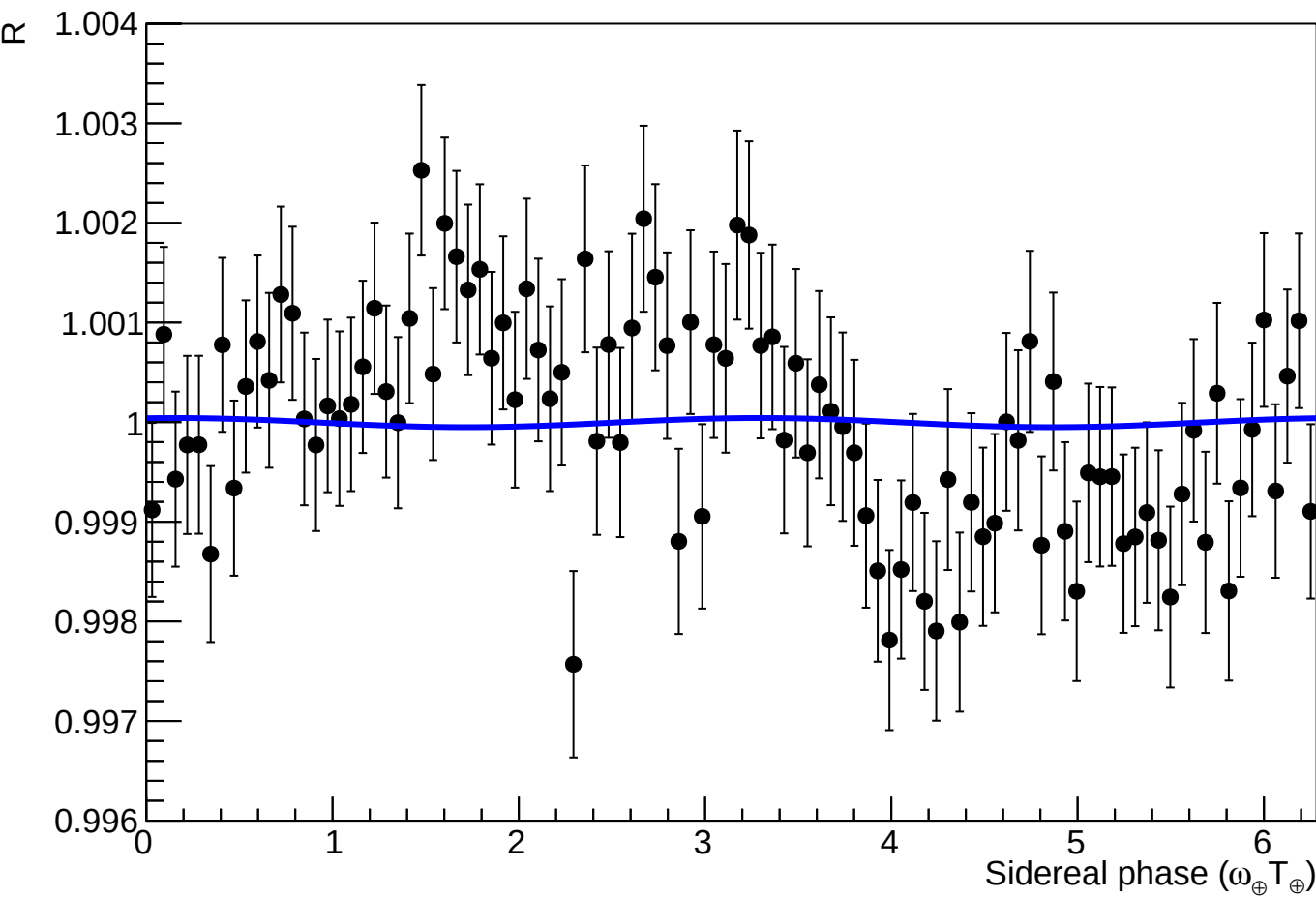
Fit to toy 37, signal shape: d2
