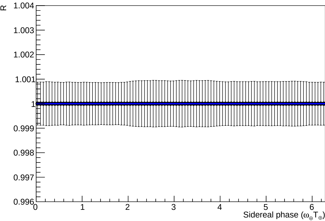
Fit to toy 36, signal shape: d3
