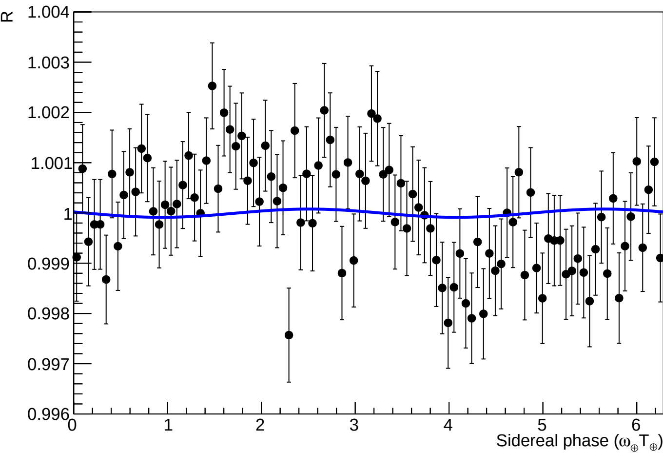
Fit to toy 37, signal shape: d3
