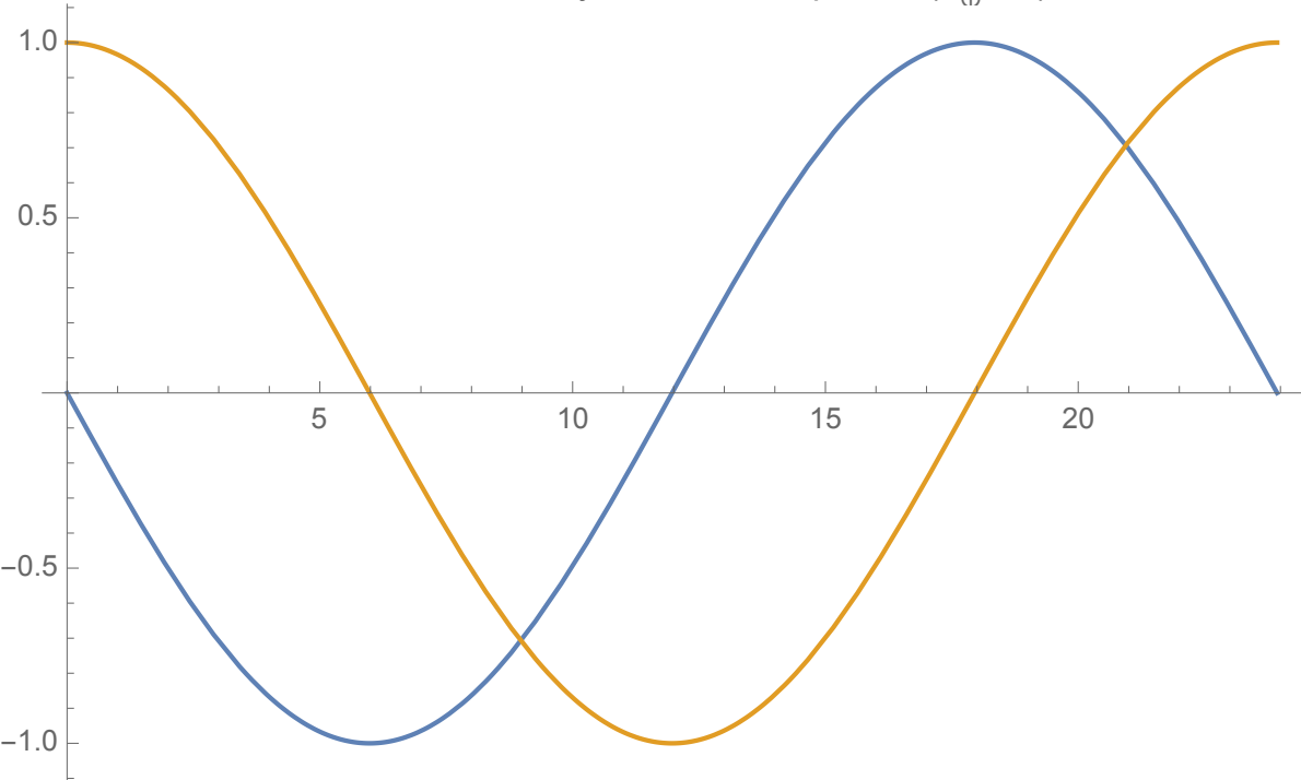
standard laboratory frame b^2 component ( T_{\oplus} = T )
