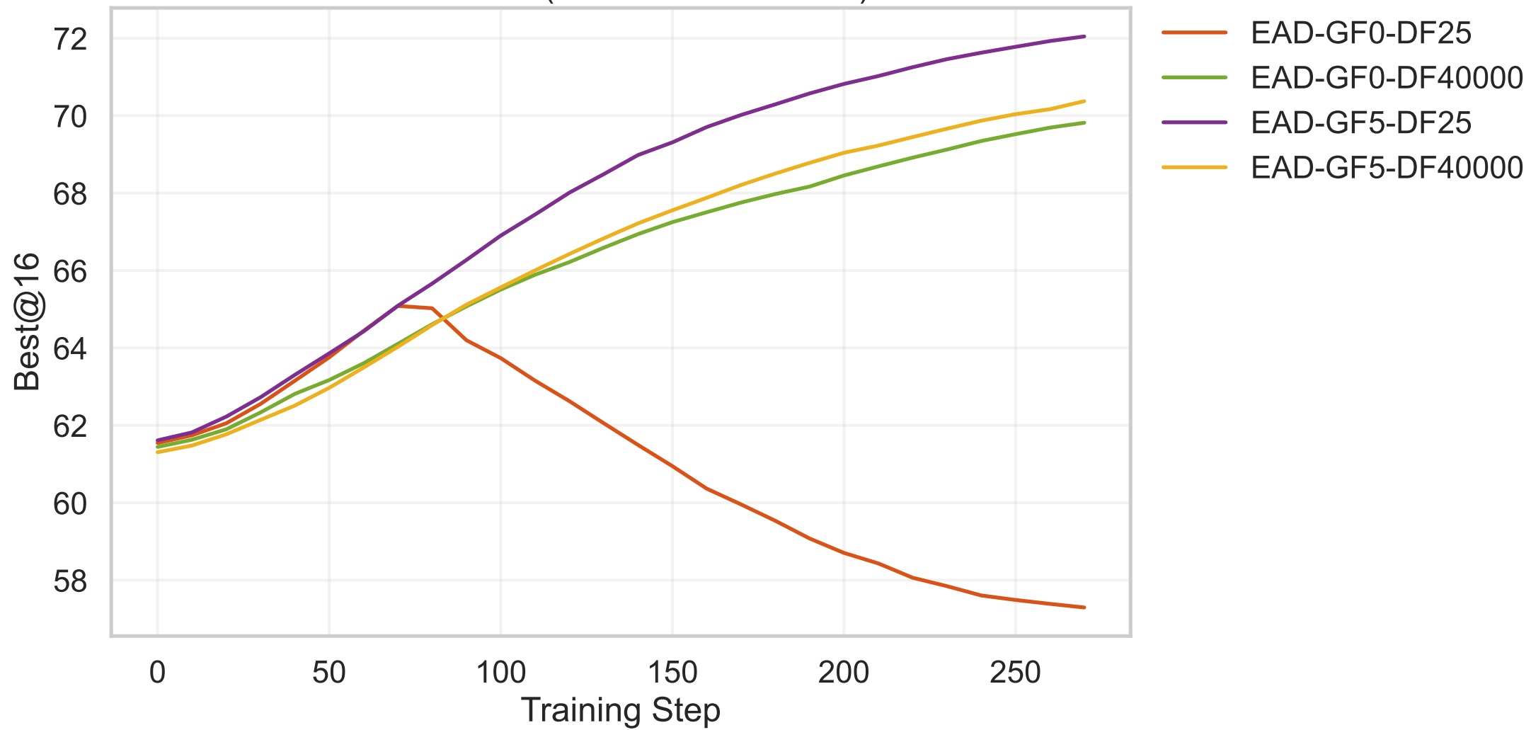
MATH-500 (Qwen2.5-Math-1.5B)
